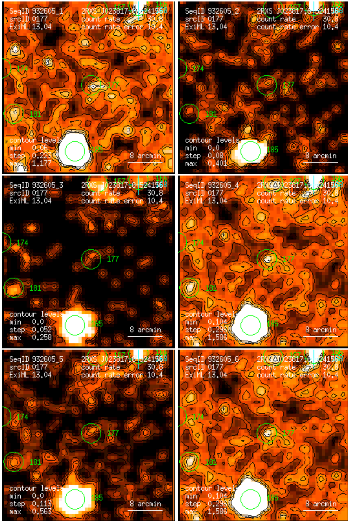
Figure 177: RASS 932605: detection 0177: band rate images, Gaussian filter: (1) PSPC channels 11 – 41, (2) 52 – 90, (3) 91 – 201, (4) 11 – 235, (5) 52 – 201, (6) 11 – 201. Broad band rates in counts/ks. Band rate contour levels in counts/ks/arcmin 2 .
