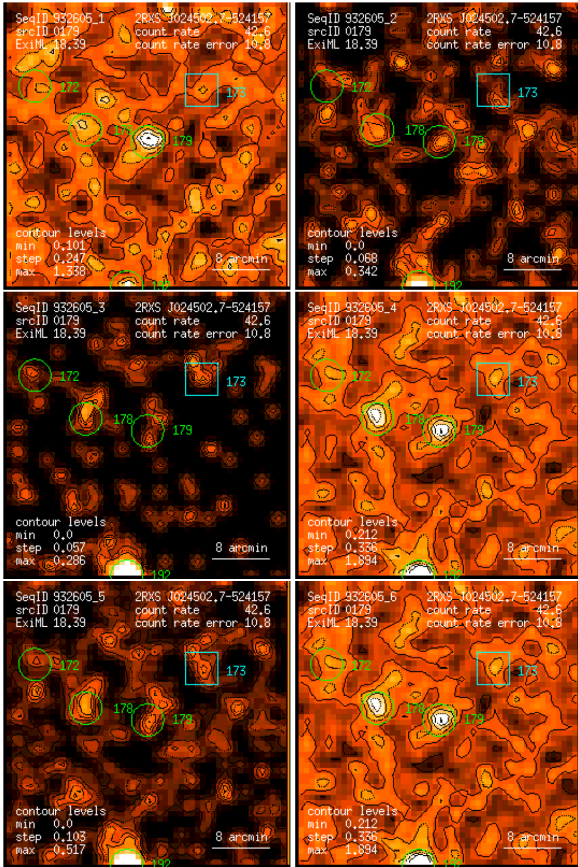
Figure 179: RASS 932605: detection 0179: band rate images, Gaussian filter: (1) PSPC channels 11 – 41, (2) 52 – 90, (3) 91 – 201, (4) 11 – 235, (5) 52 – 201, (6) 11 – 201. Broad band rates in counts/ks. Band rate contour levels in counts/ks/arcmin 2 .
