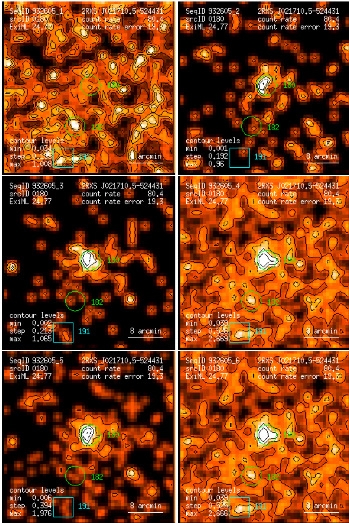
Figure 180: RASS 932605: detection 0180: band rate images, Gaussian filter: (1) PSPC channels 11 – 41, (2) 52 – 90, (3) 91 – 201, (4) 11 – 235, (5) 52 – 201, (6) 11 – 201. Broad band rates in counts/ks. Band rate contour levels in counts/ks/arcmin 2 .
