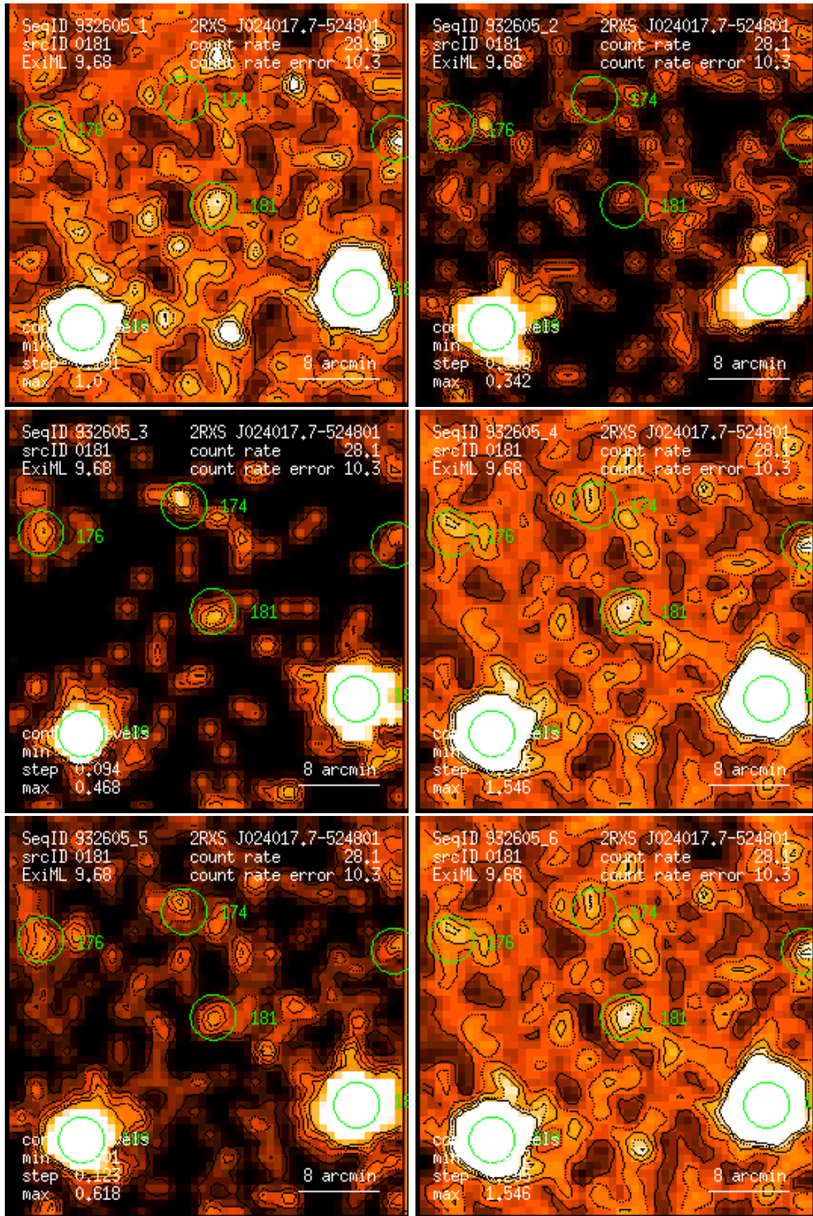
Figure 181: RASS 932605: detection 0181: band rate images, Gaussian filter: (1) PSPC channels 11 – 41, (2) 52 – 90, (3) 91 – 201, (4) 11 – 235, (5) 52 – 201, (6) 11 – 201. Broad band rates in counts/ks. Band rate contour levels in counts/ks/arcmin 2 .
