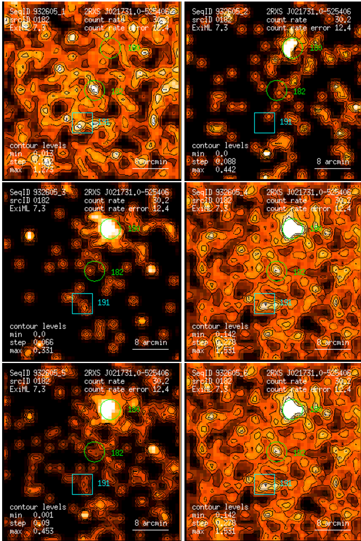
Figure 182: RASS 932605: detection 0182: band rate images, Gaussian filter: (1) PSPC channels 11 – 41, (2) 52 – 90, (3) 91 – 201, (4) 11 – 235, (5) 52 – 201, (6) 11 – 201. Broad band rates in counts/ks. Band rate contour levels in counts/ks/arcmin 2 .
