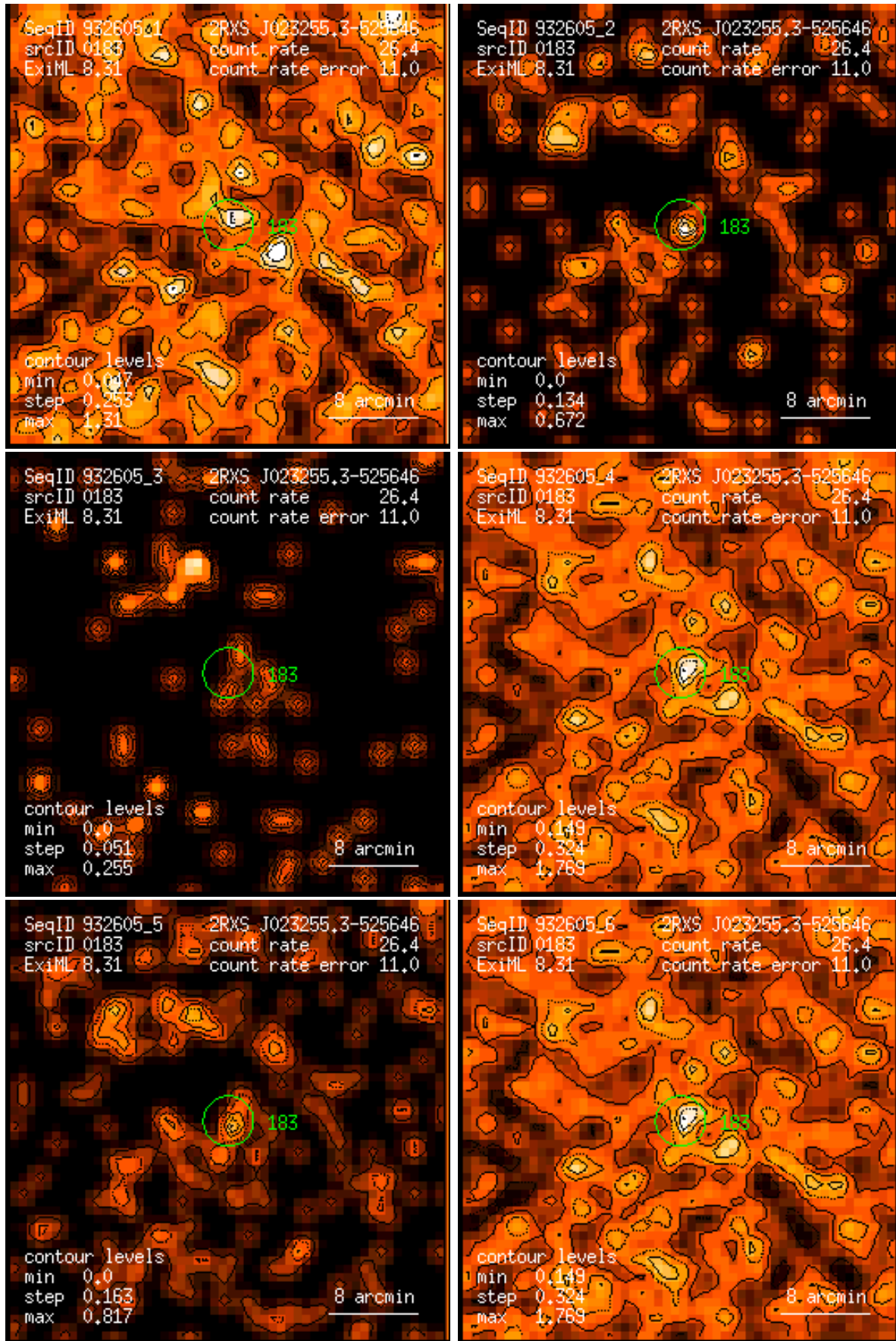
Figure 183: RASS 932605: detection 0183: band rate images, Gaussian filter: (1) PSPC channels 11 – 41, (2) 52 – 90, (3) 91 – 201, (4) 11 – 235, (5) 52 – 201, (6) 11 – 201. Broad band rates in counts/ks. Band rate contour levels in counts/ks/arcmin 2 .
