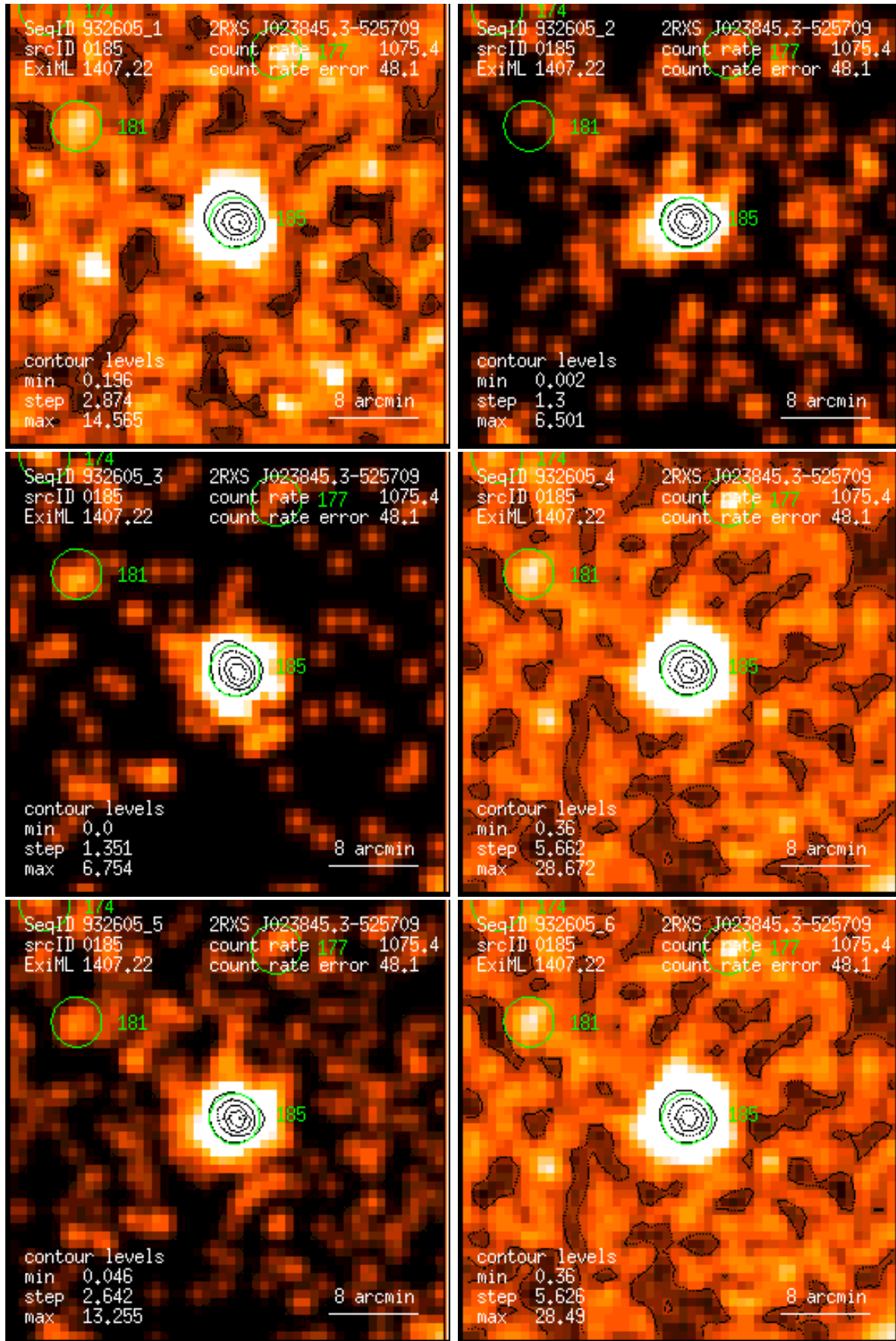
Figure 185: RASS 932605: detection 0185: band rate images, Gaussian filter: (1) PSPC channels 11 – 41, (2) 52 – 90, (3) 91 – 201, (4) 11 – 235, (5) 52 – 201, (6) 11 – 201. Broad band rates in counts/ks. Band rate contour levels in counts/ks/arcmin 2 .
