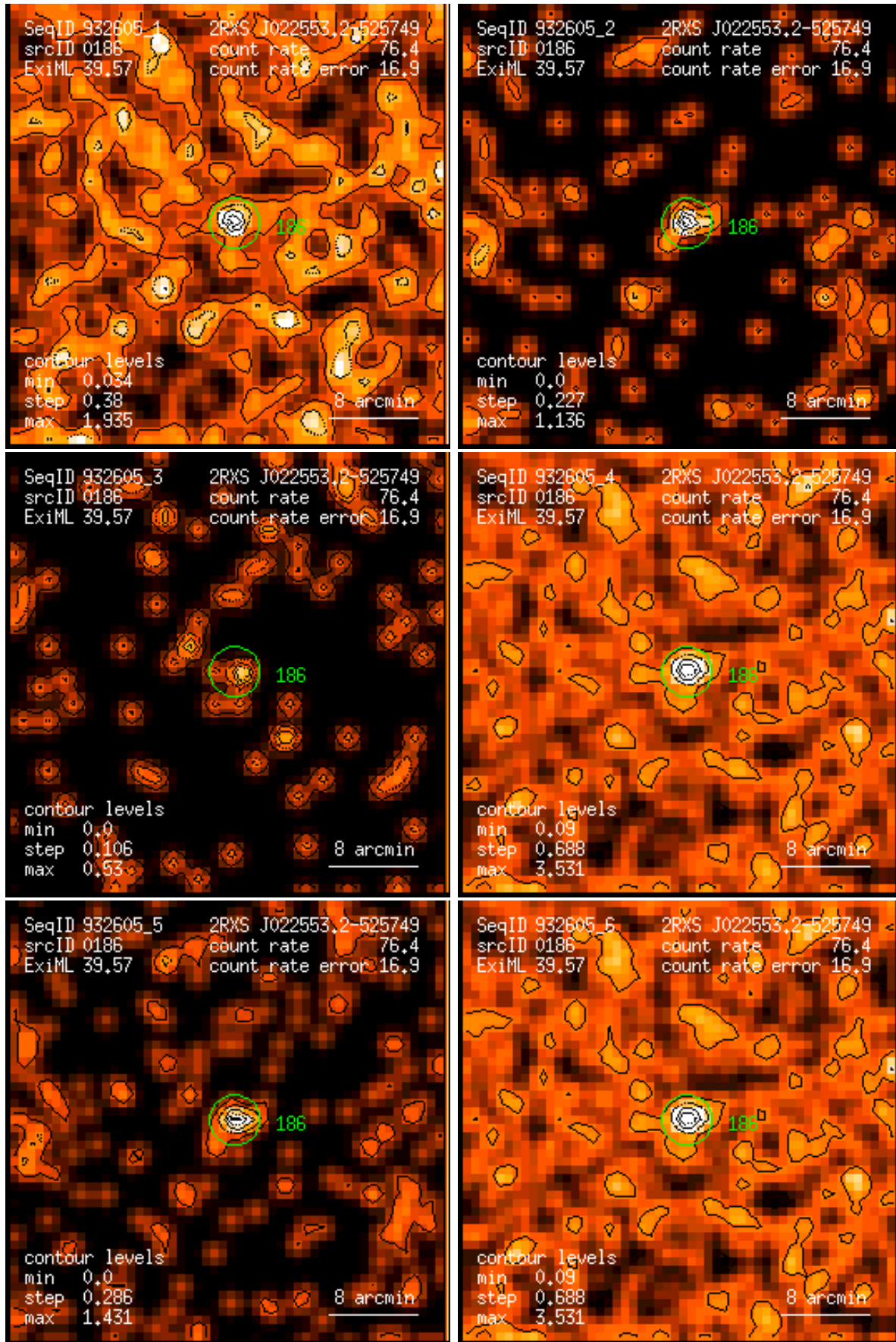
Figure 186: RASS 932605: detection 0186: band rate images, Gaussian filter: (1) PSPC channels 11 – 41, (2) 52 – 90, (3) 91 – 201, (4) 11 – 235, (5) 52 – 201, (6) 11 – 201. Broad band rates in counts/ks. Band rate contour levels in counts/ks/arcmin 2 .
