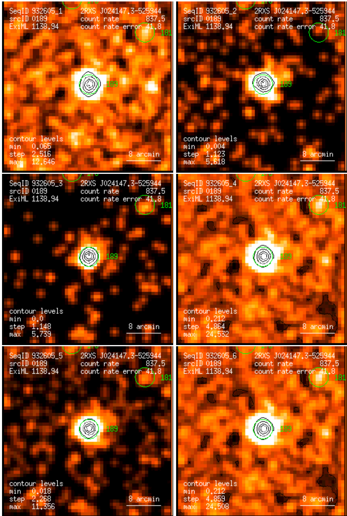
Figure 189: RASS 932605: detection 0189: band rate images, Gaussian filter: (1) PSPC channels 11 – 41, (2) 52 – 90, (3) 91 – 201, (4) 11 – 235, (5) 52 – 201, (6) 11 – 201. Broad band rates in counts/ks. Band rate contour levels in counts/ks/arcmin 2 .
