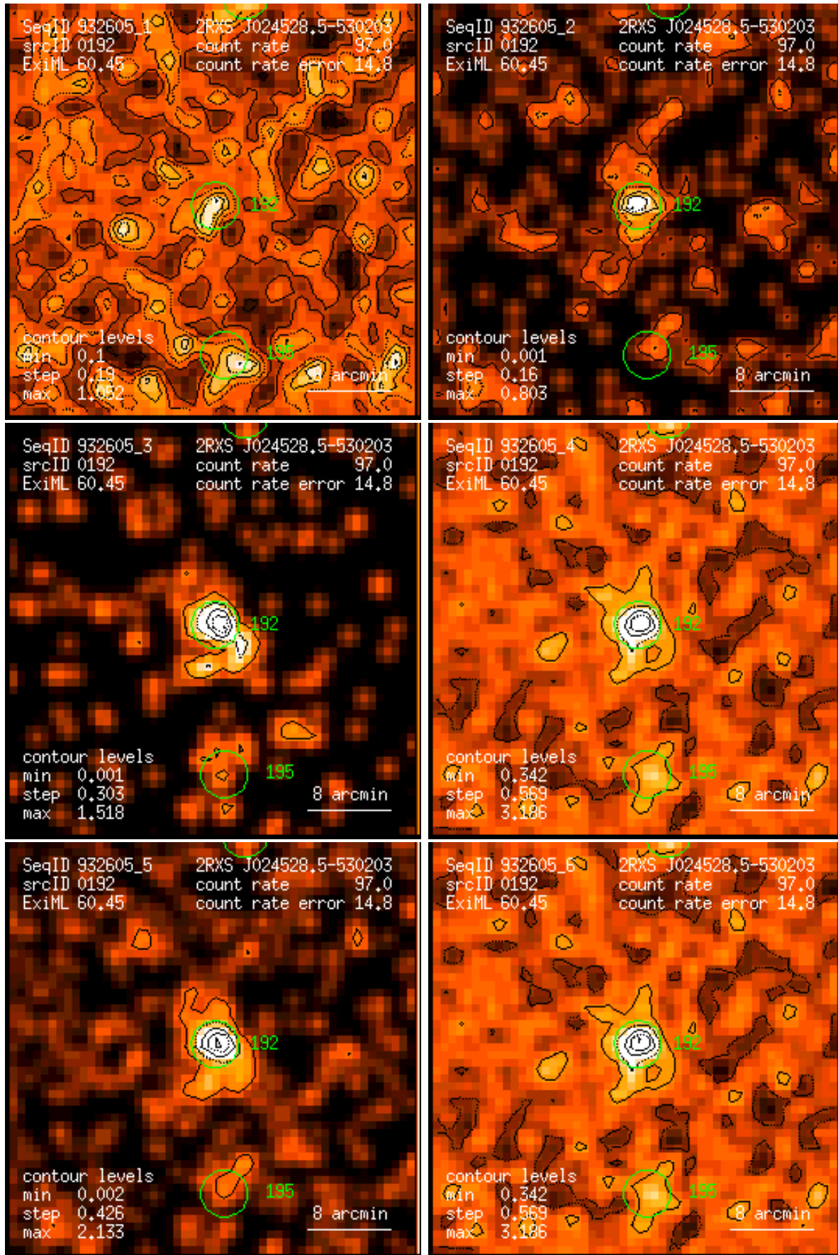
Figure 192: RASS 932605: detection 0192: band rate images, Gaussian filter: (1) PSPC channels 11 – 41, (2) 52 – 90, (3) 91 – 201, (4) 11 – 235, (5) 52 – 201, (6) 11 – 201. Broad band rates in counts/ks. Band rate contour levels in counts/ks/arcmin 2 .
