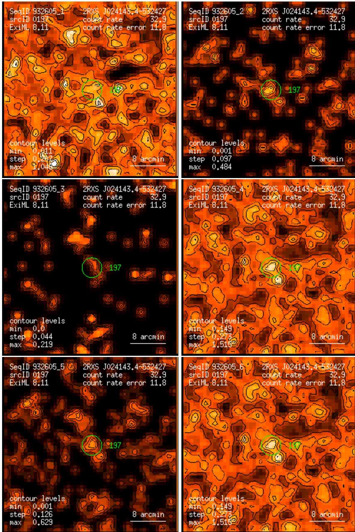
Figure 197: RASS 932605: detection 0197: band rate images, Gaussian filter: (1) PSPC channels 11 – 41, (2) 52 – 90, (3) 91 – 201, (4) 11 – 235, (5) 52 – 201, (6) 11 – 201. Broad band rates in counts/ks. Band rate contour levels in counts/ks/arcmin 2 .
