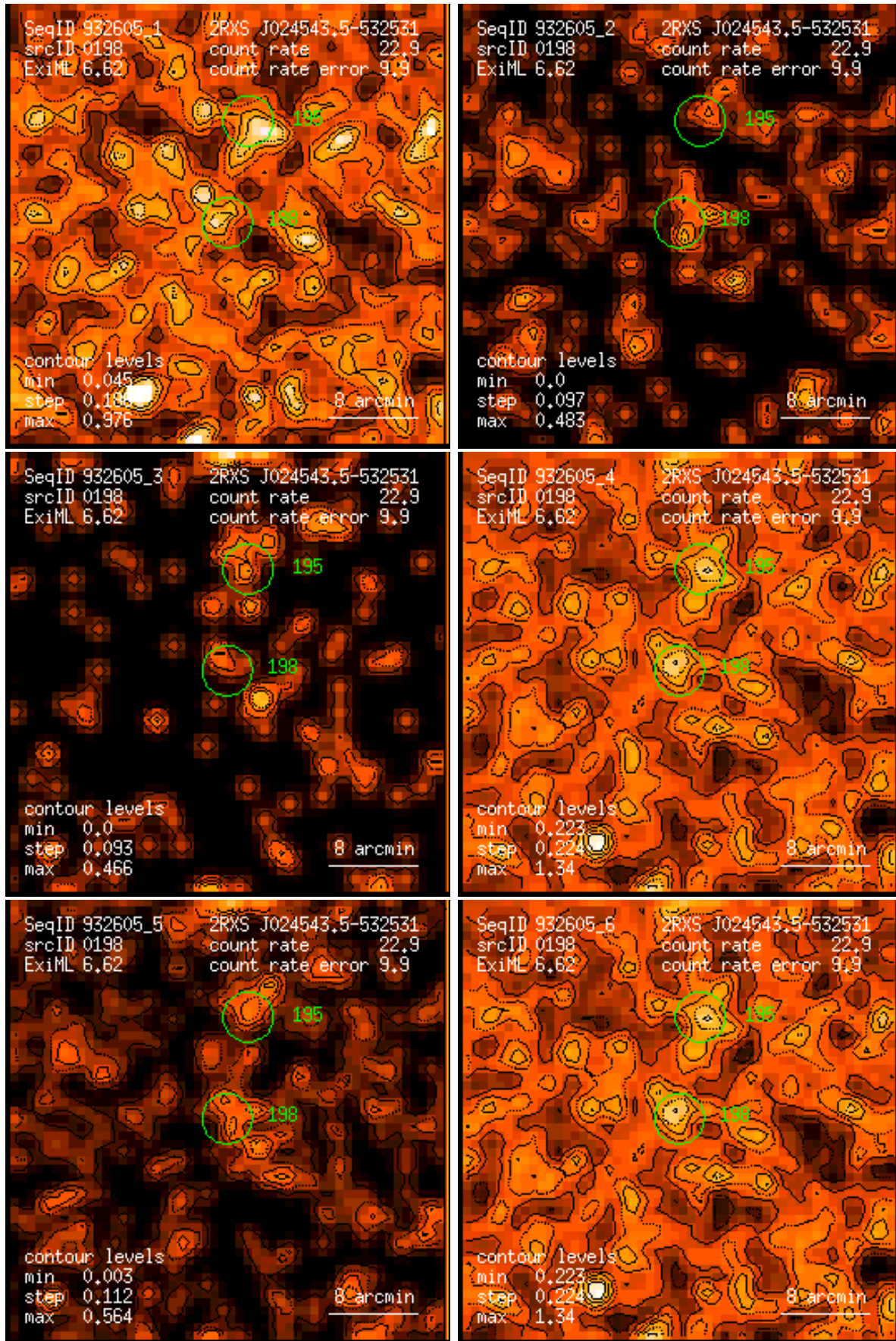
Figure 198: RASS 932605: detection 0198: band rate images, Gaussian filter: (1) PSPC channels 11 – 41, (2) 52 – 90, (3) 91 – 201, (4) 11 – 235, (5) 52 – 201, (6) 11 – 201. Broad band rates in counts/ks. Band rate contour levels in counts/ks/arcmin 2 .
