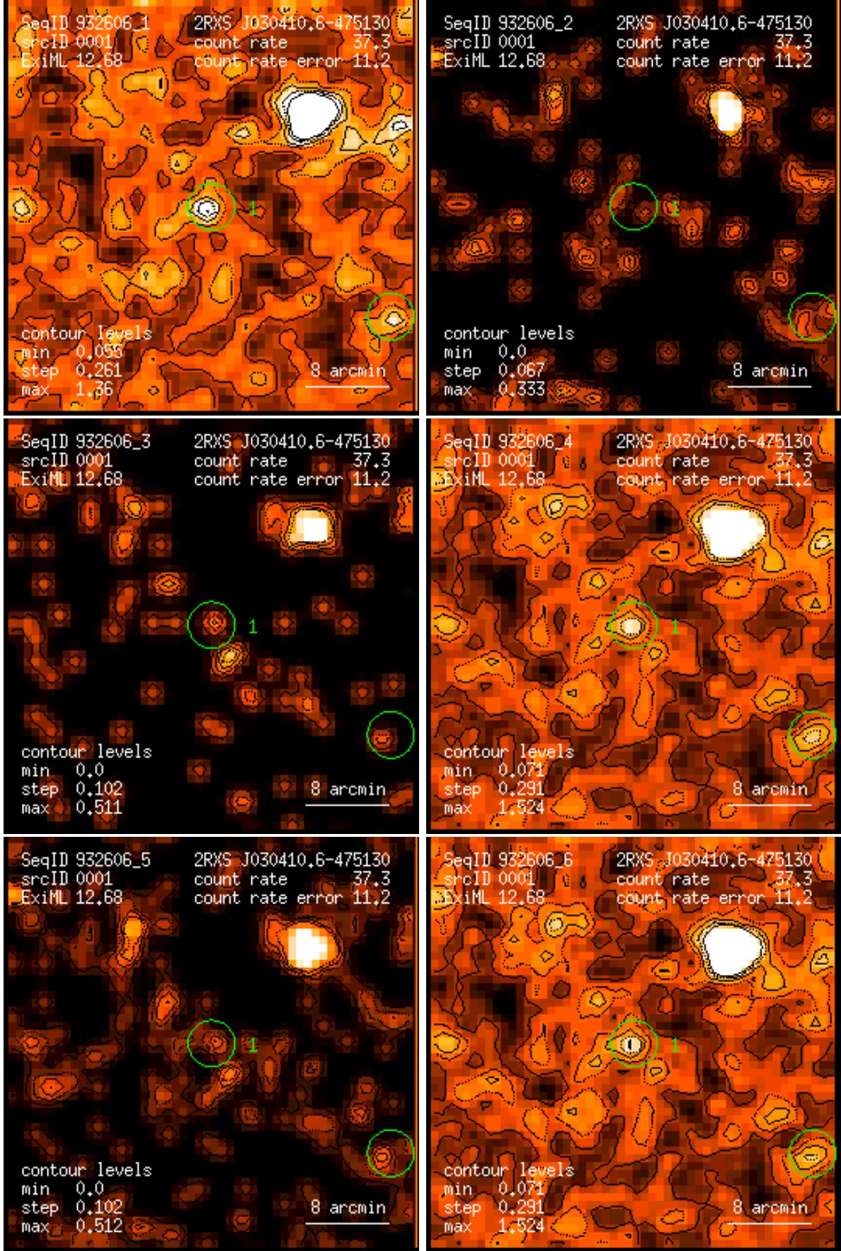
Figure 1: RASS 932606: detection 0001: band rate images, Gaussian filter: (1) PSPC channels 11 – 41, (2) 52 – 90, (3) 91 – 201, (4) 11 – 235, (5) 52 – 201, (6) 11 – 201. Broad band rates in counts/ks. Band rate contour levels in counts/ks/arcmin 2 .
