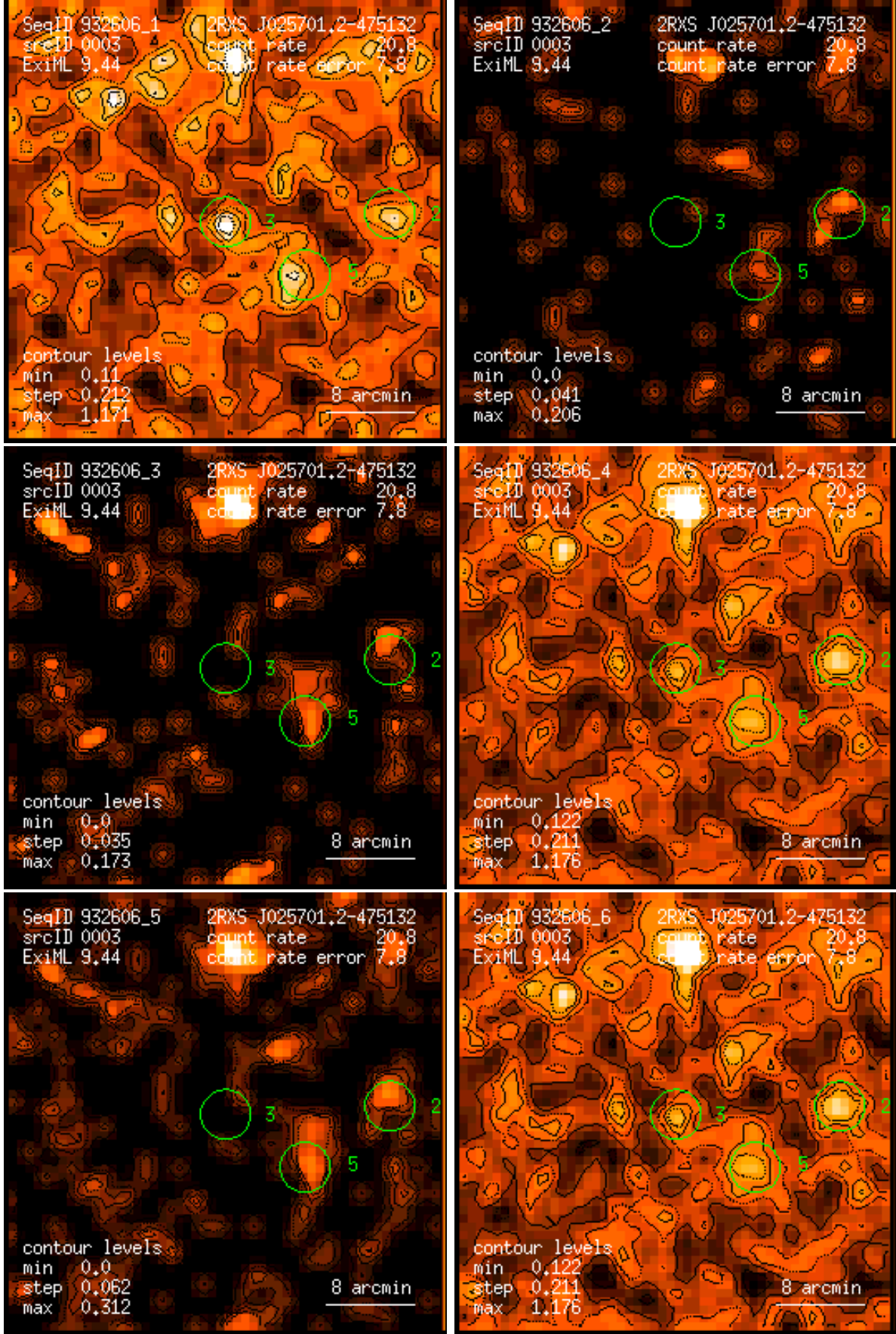
Figure 3: RASS 932606: detection 0003: band rate images, Gaussian filter: (1) PSPC channels 11 – 41, (2) 52 – 90, (3) 91 – 201, (4) 11 – 235, (5) 52 – 201, (6) 11 – 201. Broad band rates in counts/ks. Band rate contour levels in counts/ks/arcmin 2 .
