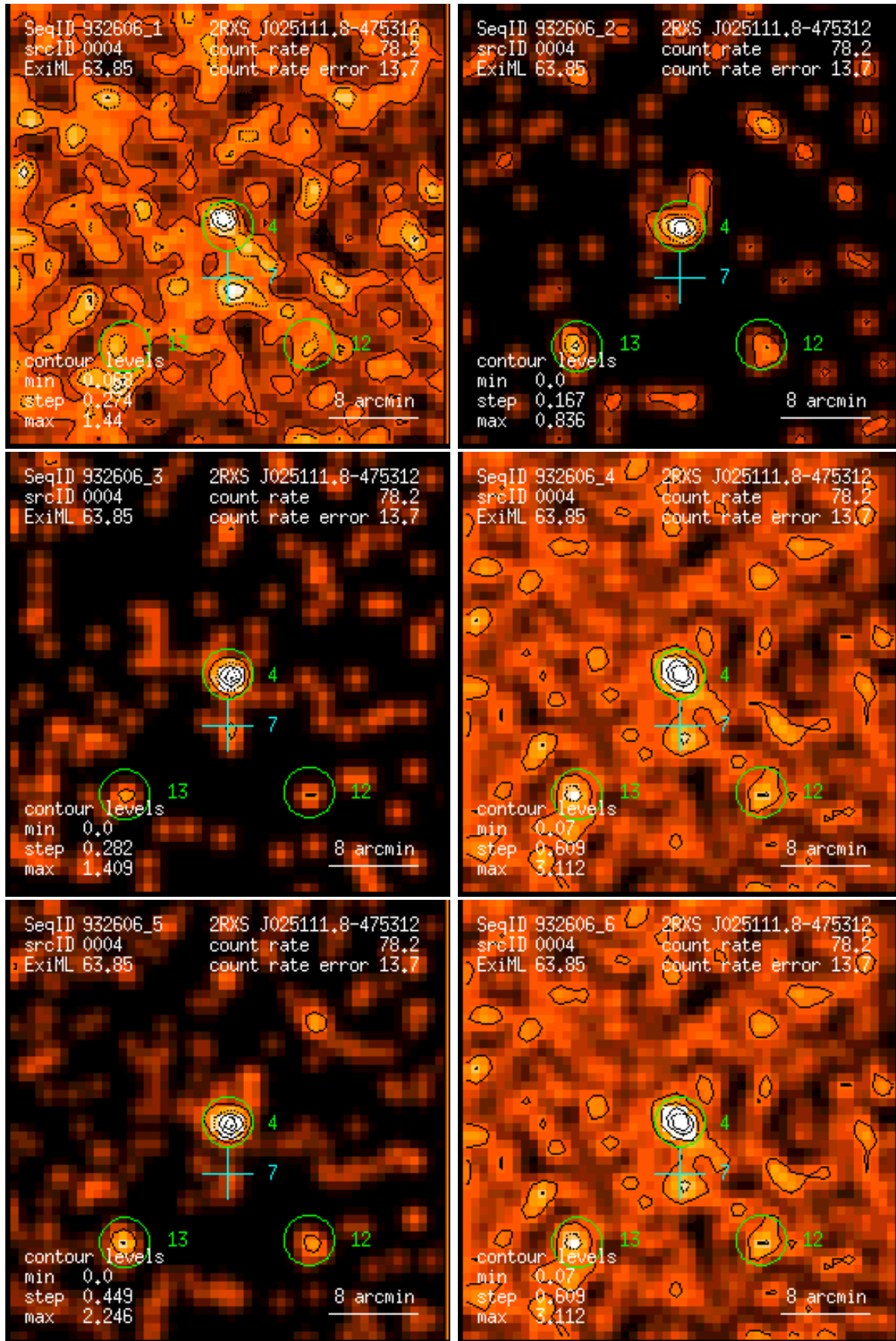
Figure 4: RASS 932606: detection 0004: band rate images, Gaussian filter: (1) PSPC channels 11 – 41, (2) 52 – 90, (3) 91 – 201, (4) 11 – 235, (5) 52 – 201, (6) 11 – 201. Broad band rates in counts/ks. Band rate contour levels in counts/ks/arcmin 2 .
