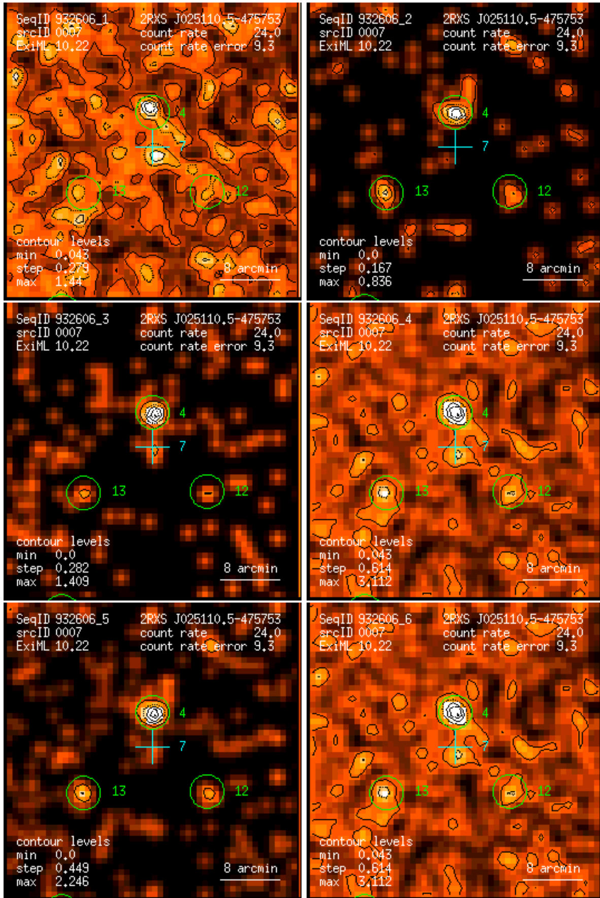
Figure 7: RASS 932606: detection 0007: band rate images, Gaussian filter: (1) PSPC channels 11 – 41, (2) 52 – 90, (3) 91 – 201, (4) 11 – 235, (5) 52 – 201, (6) 11 – 201. Broad band rates in counts/ks. Band rate contour levels in counts/ks/arcmin 2 .
