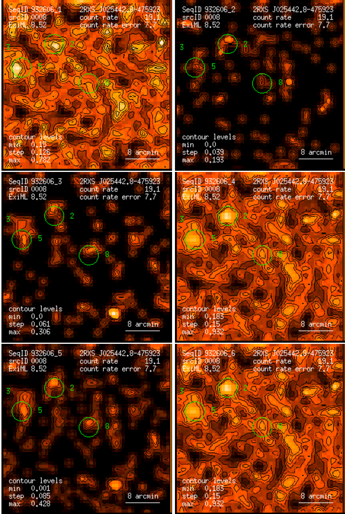
Figure 8: RASS 932606: detection 0008: band rate images, Gaussian filter: (1) PSPC channels 11 – 41, (2) 52 – 90, (3) 91 – 201, (4) 11 – 235, (5) 52 – 201, (6) 11 – 201. Broad band rates in counts/ks. Band rate contour levels in counts/ks/arcmin 2 .
