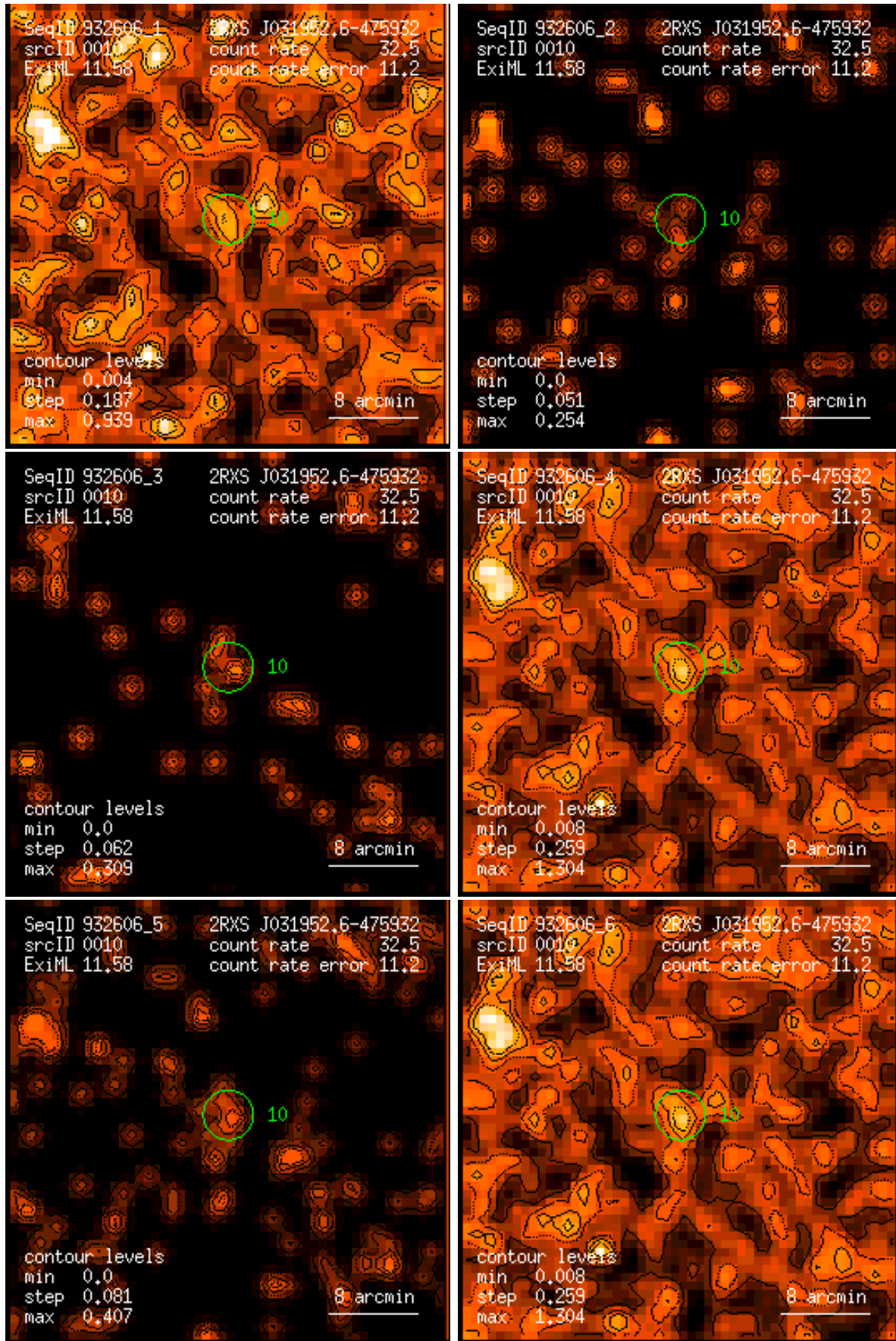
Figure 10: RASS 932606: detection 0010: band rate images, Gaussian filter: (1) PSPC channels 11 – 41, (2) 52 – 90, (3) 91 – 201, (4) 11 – 235, (5) 52 – 201, (6) 11 – 201. Broad band rates in counts/ks. Band rate contour levels in counts/ks/arcmin 2 .
