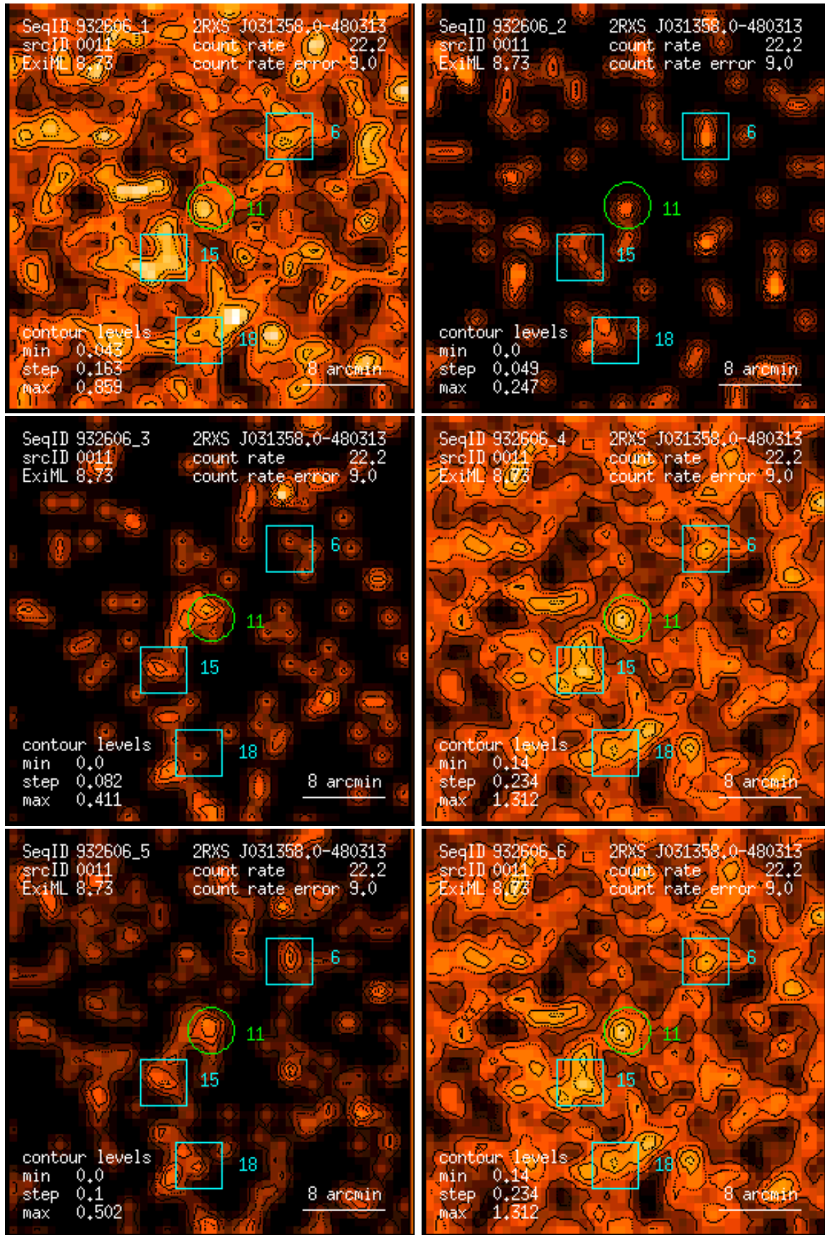
Figure 11: RASS 932606: detection 0011: band rate images, Gaussian filter: (1) PSPC channels 11 – 41, (2) 52 – 90, (3) 91 – 201, (4) 11 – 235, (5) 52 – 201, (6) 11 – 201. Broad band rates in counts/ks. Band rate contour levels in counts/ks/arcmin 2 .
