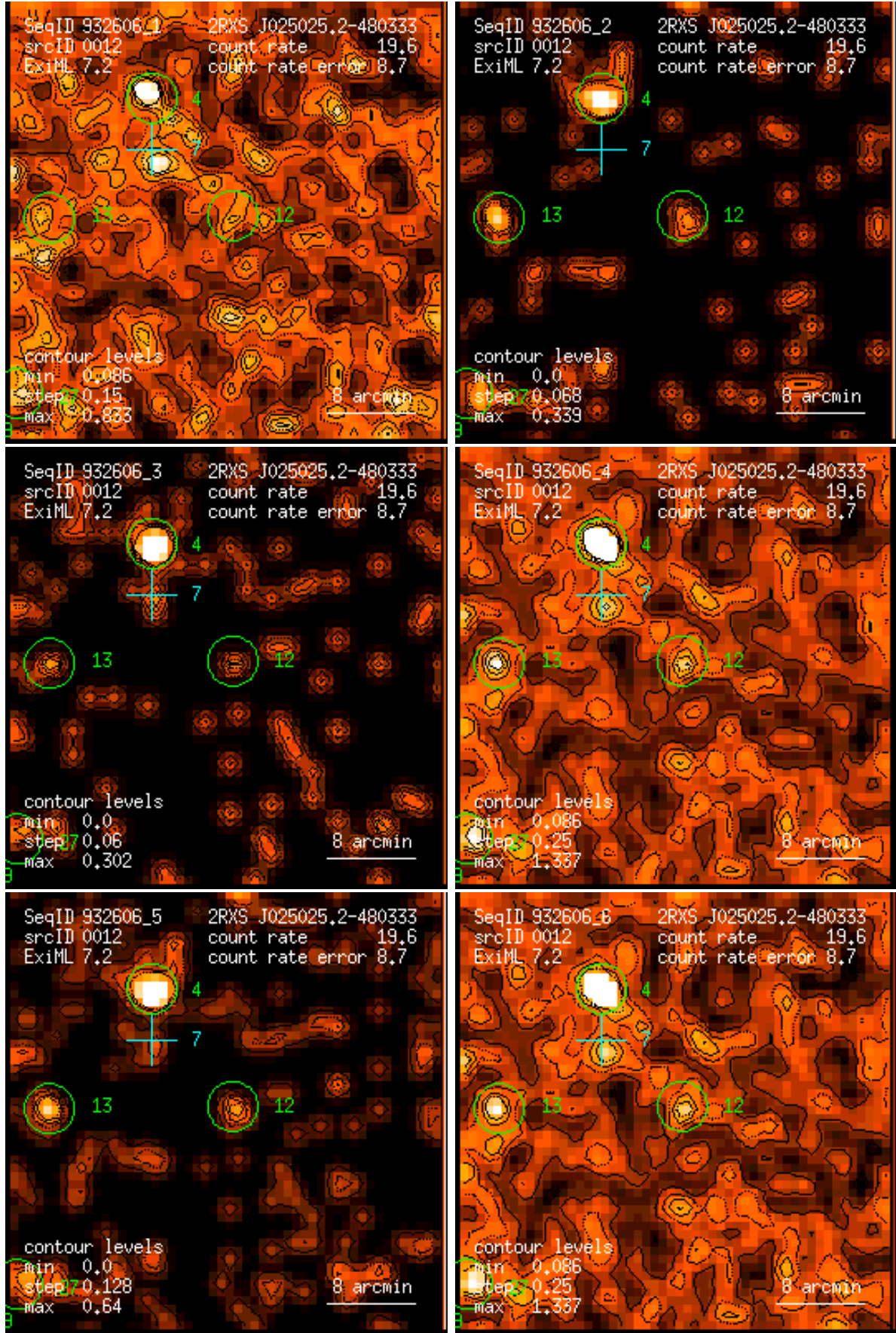
Figure 12: RASS 932606: detection 0012: band rate images, Gaussian filter: (1) PSPC channels 11 – 41, (2) 52 – 90, (3) 91 – 201, (4) 11 – 235, (5) 52 – 201, (6) 11 – 201. Broad band rates in counts/ks. Band rate contour levels in counts/ks/arcmin 2 .
