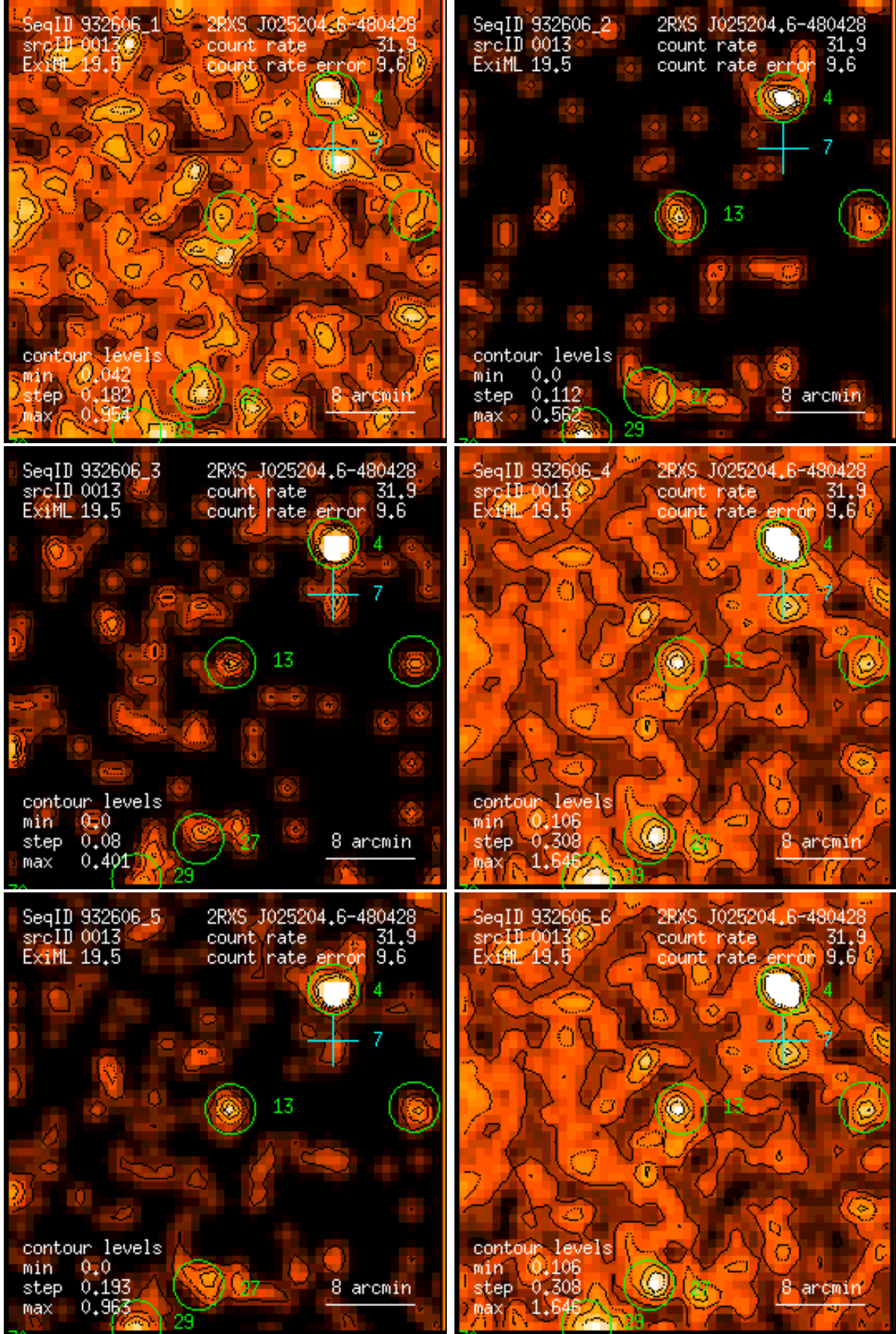
Figure 13: RASS 932606: detection 0013: band rate images, Gaussian filter: (1) PSPC channels 11 – 41, (2) 52 – 90, (3) 91 – 201, (4) 11 – 235, (5) 52 – 201, (6) 11 – 201. Broad band rates in counts/ks. Band rate contour levels in counts/ks/arcmin 2 .
