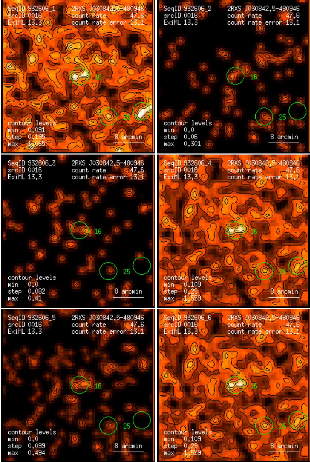
Figure 16: RASS 932606: detection 0016: band rate images, Gaussian filter: (1) PSPC channels 11 – 41, (2) 52 – 90, (3) 91 – 201, (4) 11 – 235, (5) 52 – 201, (6) 11 – 201. Broad band rates in counts/ks. Band rate contour levels in counts/ks/arcmin 2 .
