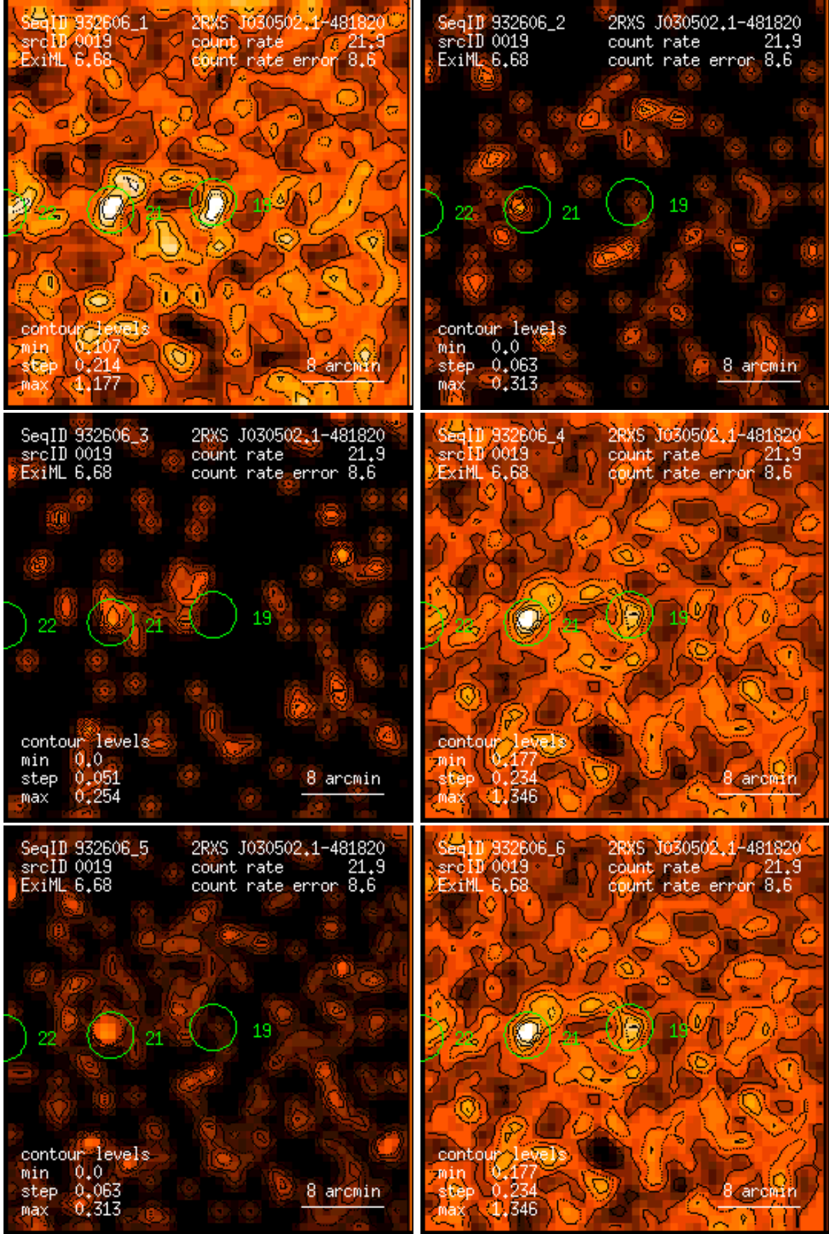
Figure 19: RASS 932606: detection 0019: band rate images, Gaussian filter: (1) PSPC channels 11 – 41, (2) 52 – 90, (3) 91 – 201, (4) 11 – 235, (5) 52 – 201, (6) 11 – 201. Broad band rates in counts/ks. Band rate contour levels in counts/ks/arcmin 2 .
