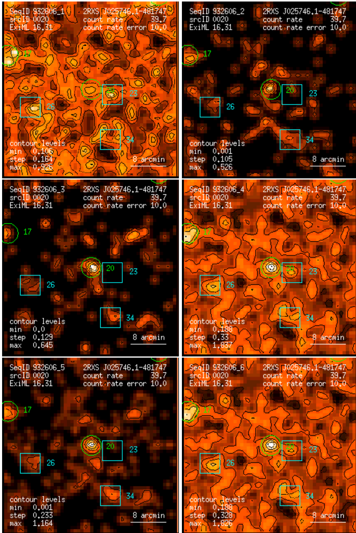
Figure 20: RASS 932606: detection 0020: band rate images, Gaussian filter: (1) PSPC channels 11 – 41, (2) 52 – 90, (3) 91 – 201, (4) 11 – 235, (5) 52 – 201, (6) 11 – 201. Broad band rates in counts/ks. Band rate contour levels in counts/ks/arcmin 2 .
