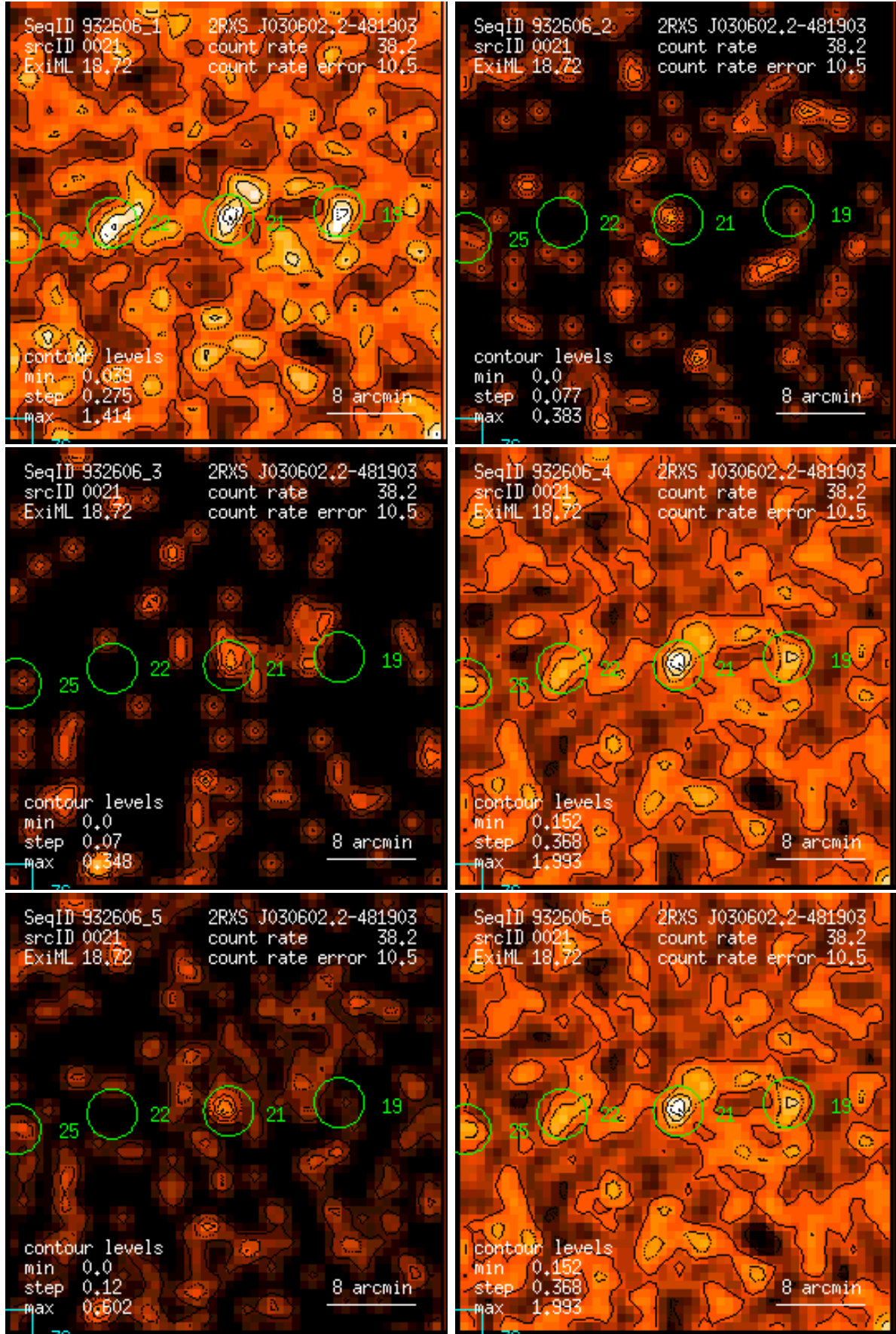
Figure 21: RASS 932606: detection 0021: band rate images, Gaussian filter: (1) PSPC channels 11 – 41, (2) 52 – 90, (3) 91 – 201, (4) 11 – 235, (5) 52 – 201, (6) 11 – 201. Broad band rates in counts/ks. Band rate contour levels in counts/ks/arcmin 2 .
