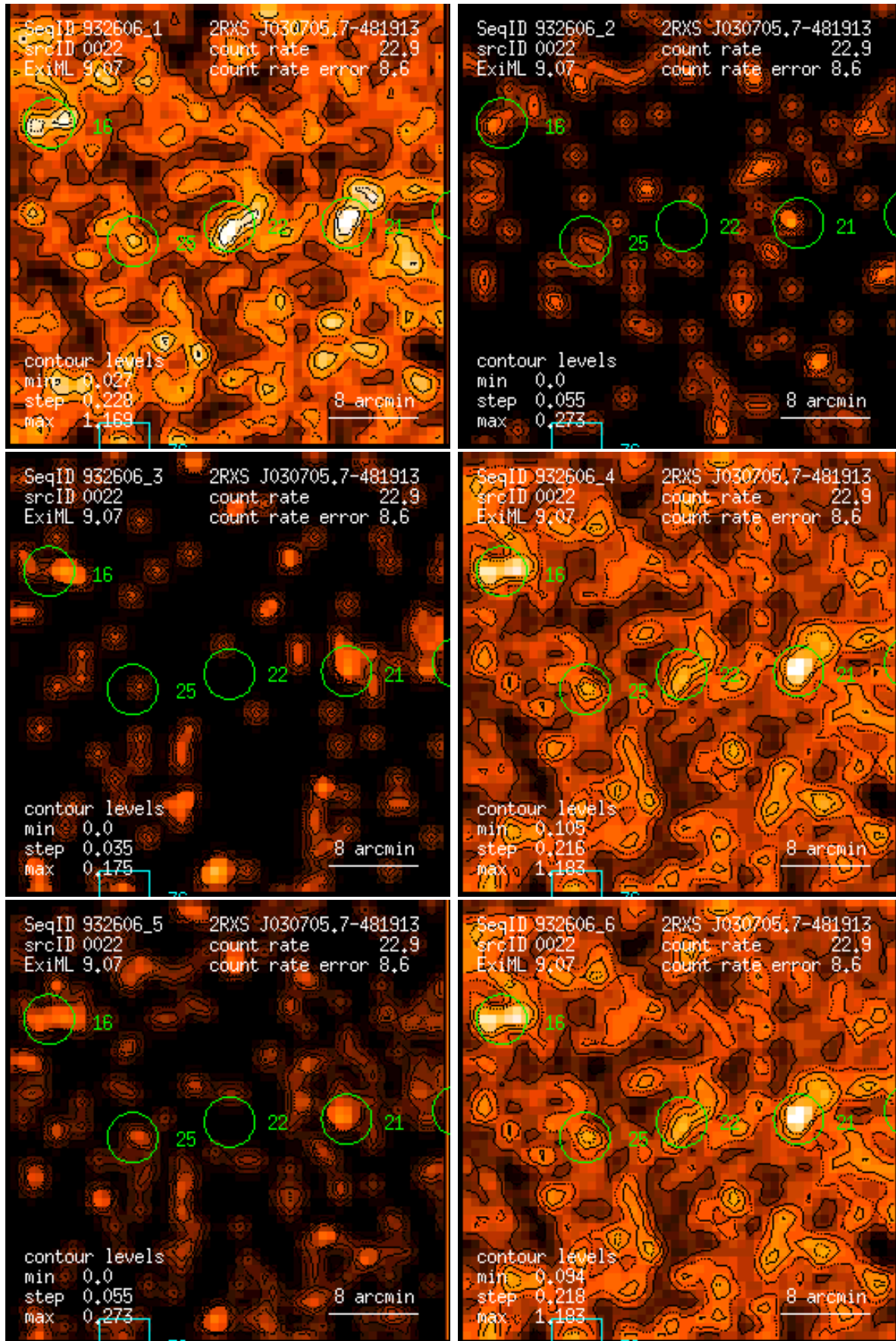
Figure 22: RASS 932606: detection 0022: band rate images, Gaussian filter: (1) PSPC channels 11 – 41, (2) 52 – 90, (3) 91 – 201, (4) 11 – 235, (5) 52 – 201, (6) 11 – 201. Broad band rates in counts/ks. Band rate contour levels in counts/ks/arcmin 2 .
