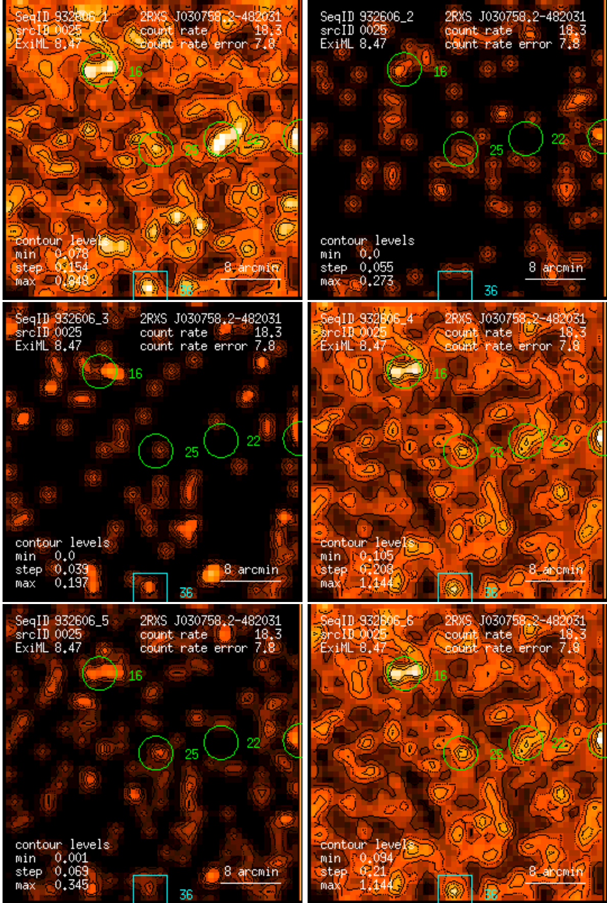
Figure 25: RASS 932606: detection 0025: band rate images, Gaussian filter: (1) PSPC channels 11 – 41, (2) 52 – 90, (3) 91 – 201, (4) 11 – 235, (5) 52 – 201, (6) 11 – 201. Broad band rates in counts/ks. Band rate contour levels in counts/ks/arcmin 2 .
