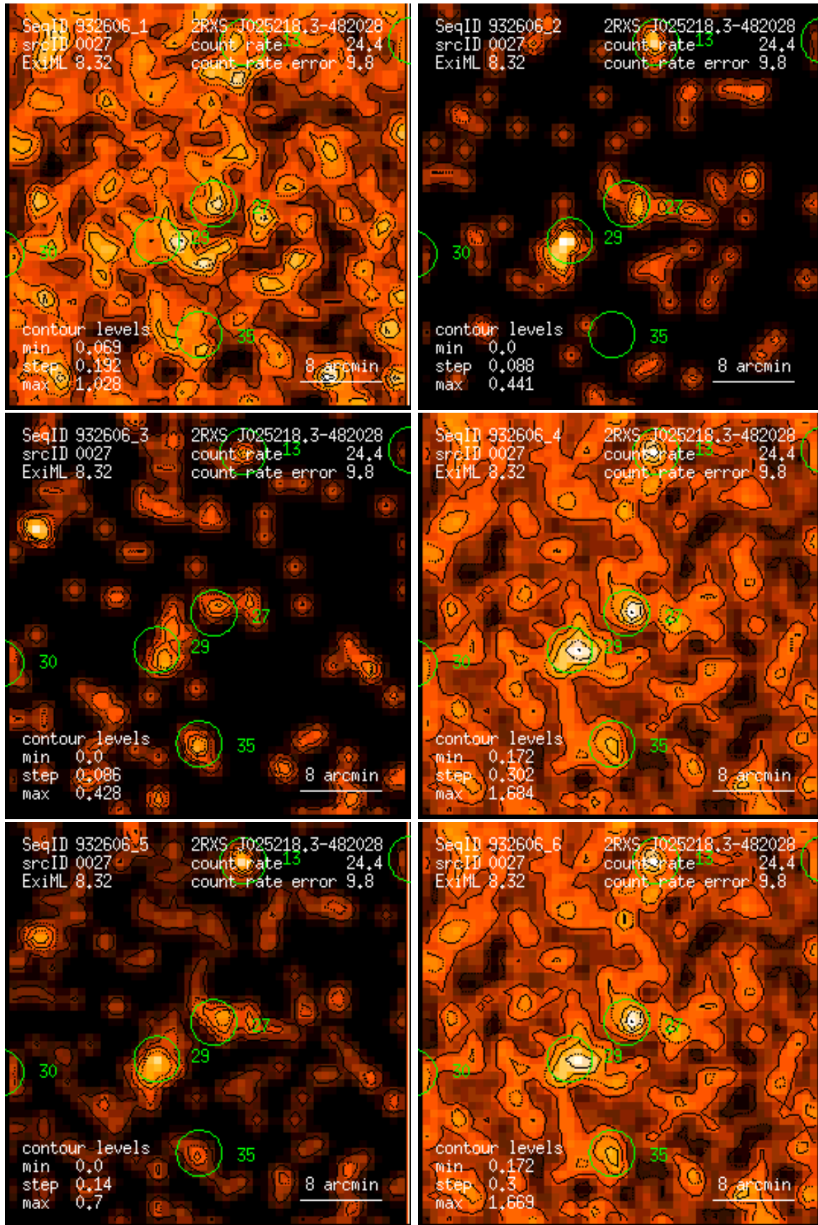
Figure 27: RASS 932606: detection 0027: band rate images, Gaussian filter: (1) PSPC channels 11 – 41, (2) 52 – 90, (3) 91 – 201, (4) 11 – 235, (5) 52 – 201, (6) 11 – 201. Broad band rates in counts/ks. Band rate contour levels in counts/ks/arcmin 2 .
