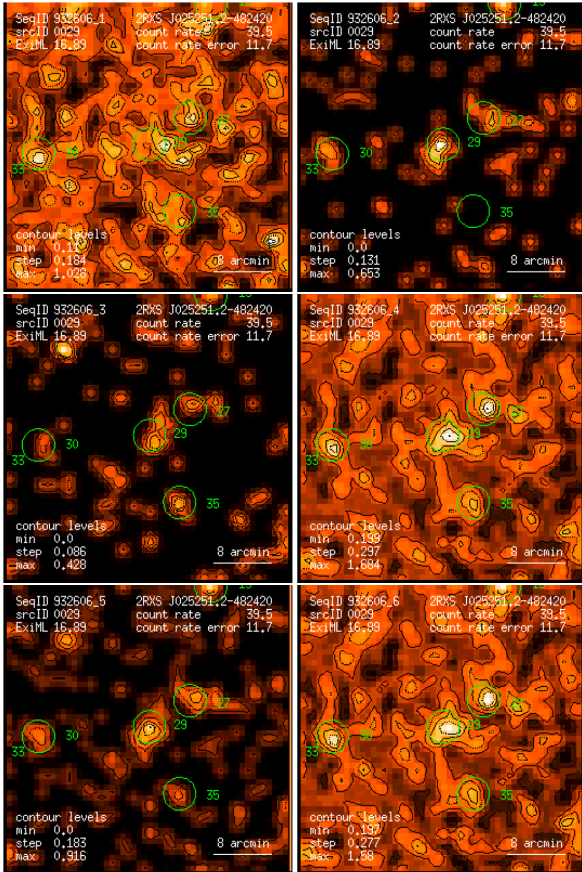
Figure 29: RASS 932606: detection 0029: band rate images, Gaussian filter: (1) PSPC channels 11 – 41, (2) 52 – 90, (3) 91 – 201, (4) 11 – 235, (5) 52 – 201, (6) 11 – 201. Broad band rates in counts/ks. Band rate contour levels in counts/ks/arcmin 2 .
