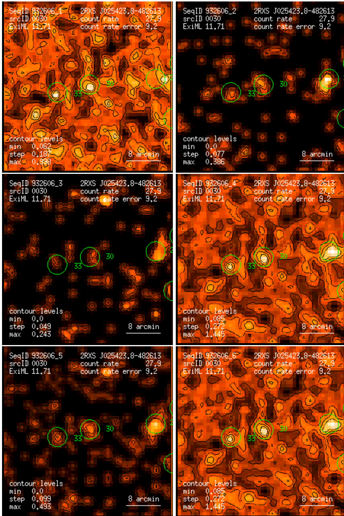
Figure 30: RASS 932606: detection 0030: band rate images, Gaussian filter: (1) PSPC channels 11 – 41, (2) 52 – 90, (3) 91 – 201, (4) 11 – 235, (5) 52 – 201, (6) 11 – 201. Broad band rates in counts/ks. Band rate contour levels in counts/ks/arcmin 2 .
