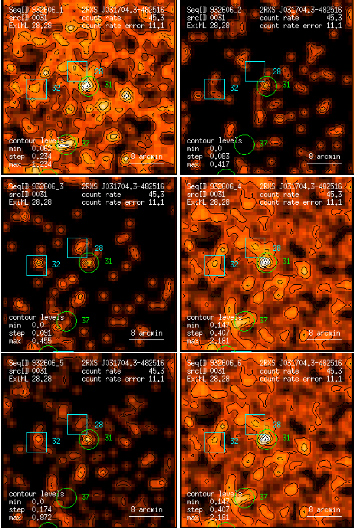
Figure 31: RASS 932606: detection 0031: band rate images, Gaussian filter: (1) PSPC channels 11 – 41, (2) 52 – 90, (3) 91 – 201, (4) 11 – 235, (5) 52 – 201, (6) 11 – 201. Broad band rates in counts/ks. Band rate contour levels in counts/ks/arcmin 2 .
