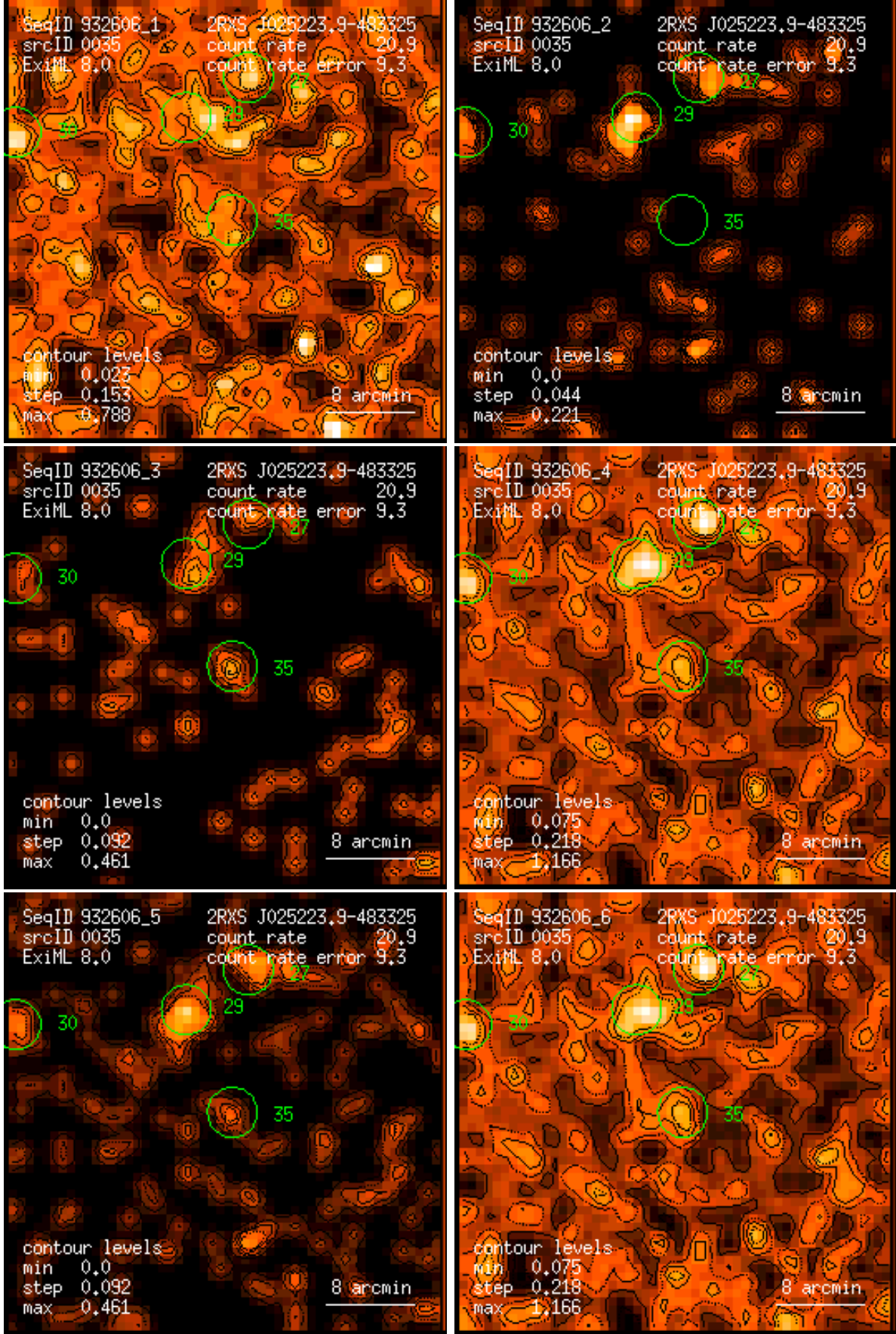
Figure 35: RASS 932606: detection 0035: band rate images, Gaussian filter: (1) PSPC channels 11 – 41, (2) 52 – 90, (3) 91 – 201, (4) 11 – 235, (5) 52 – 201, (6) 11 – 201. Broad band rates in counts/ks. Band rate contour levels in counts/ks/arcmin 2 .
