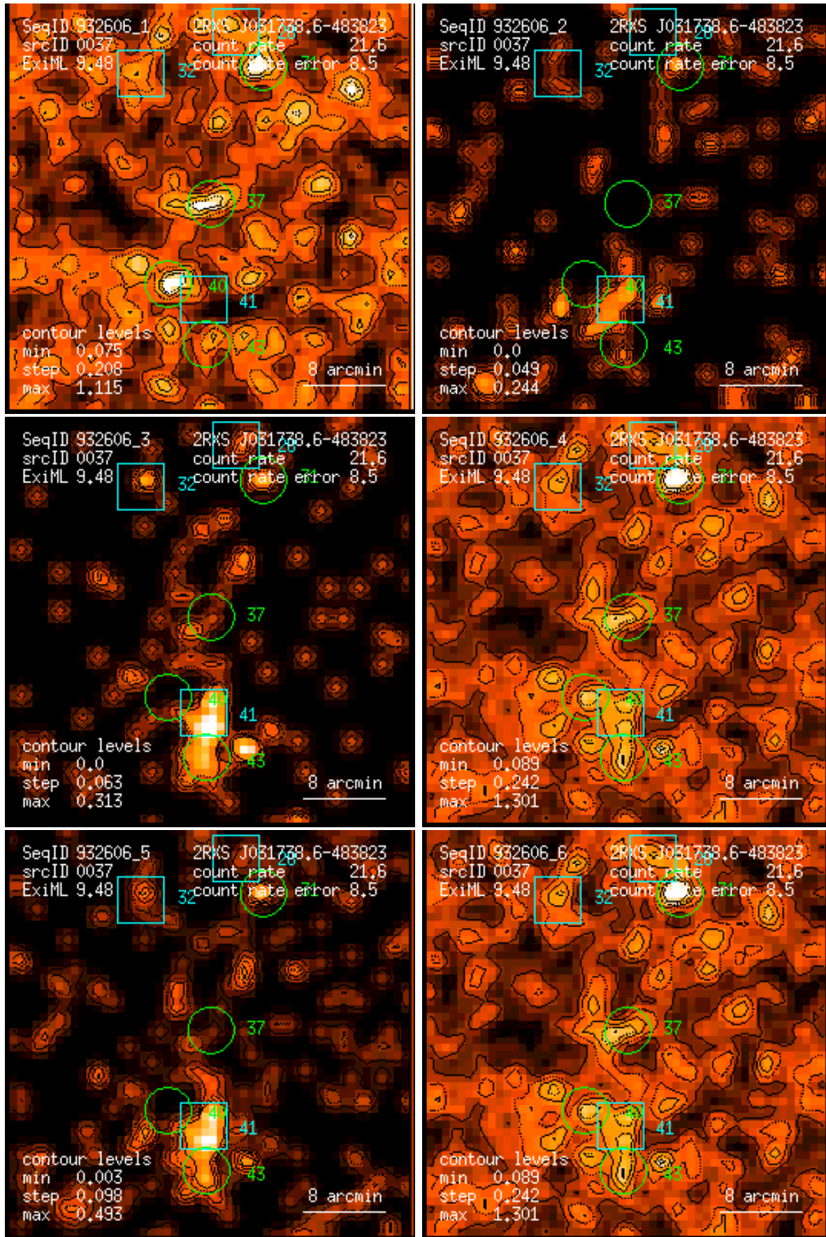
Figure 37: RASS 932606: detection 0037: band rate images, Gaussian filter: (1) PSPC channels 11 – 41, (2) 52 – 90, (3) 91 – 201, (4) 11 – 235, (5) 52 – 201, (6) 11 – 201. Broad band rates in counts/ks. Band rate contour levels in counts/ks/arcmin 2 .
