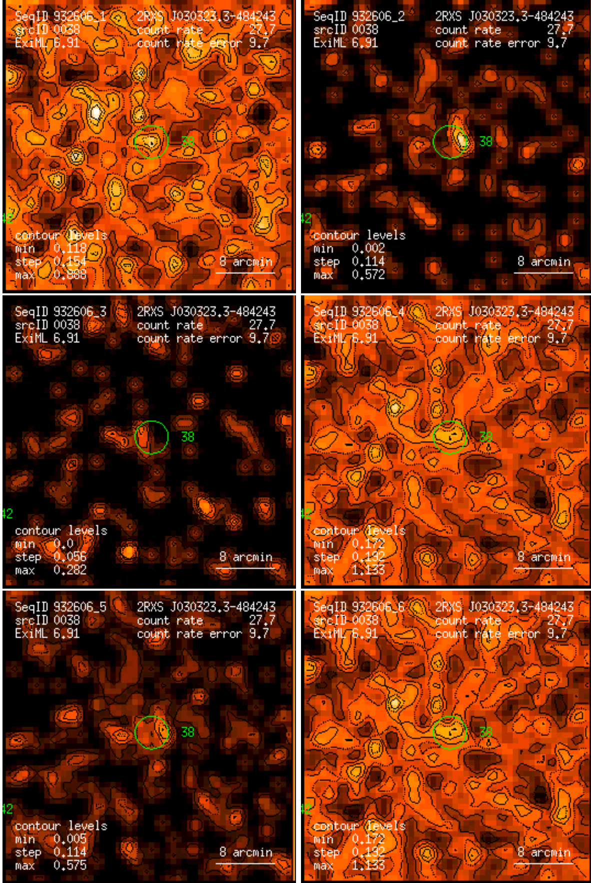
Figure 38: RASS 932606: detection 0038: band rate images, Gaussian filter: (1) PSPC channels 11 – 41, (2) 52 – 90, (3) 91 – 201, (4) 11 – 235, (5) 52 – 201, (6) 11 – 201. Broad band rates in counts/ks. Band rate contour levels in counts/ks/arcmin 2 .
