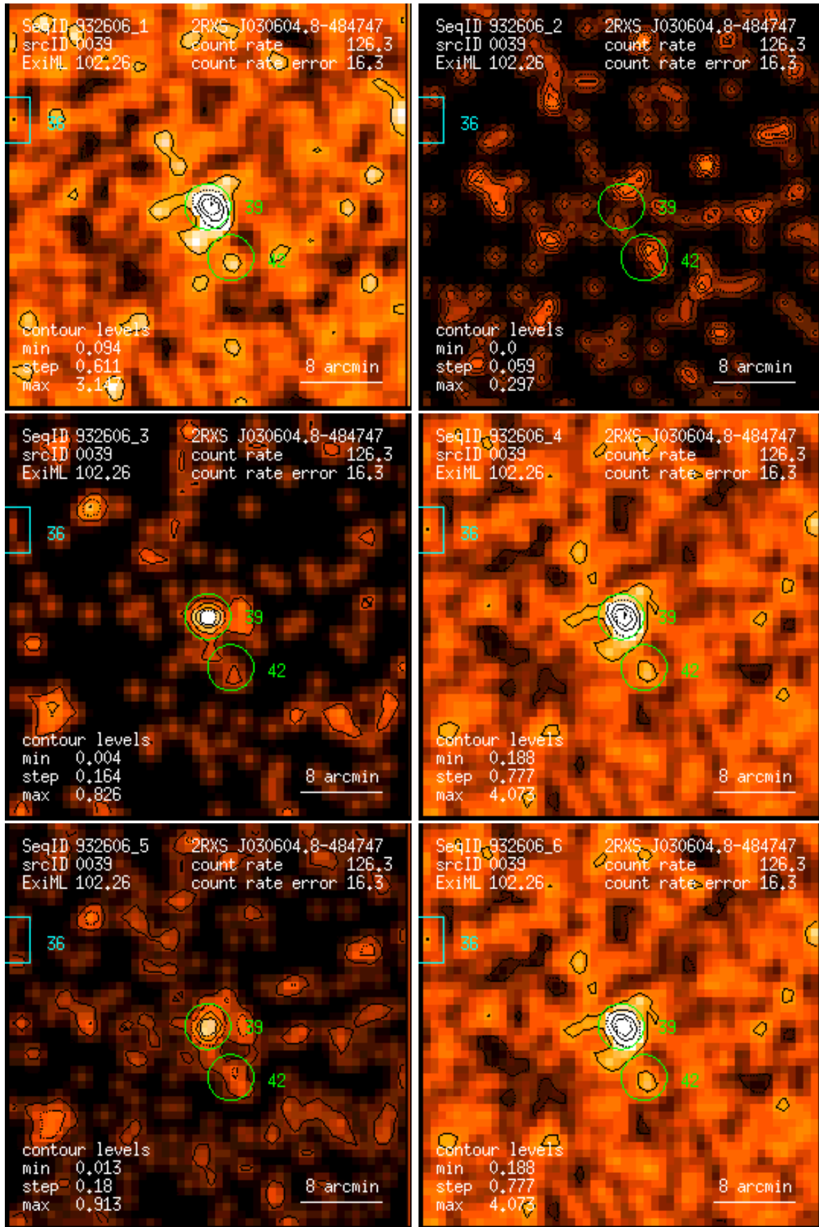
Figure 39: RASS 932606: detection 0039: band rate images, Gaussian filter: (1) PSPC channels 11 – 41, (2) 52 – 90, (3) 91 – 201, (4) 11 – 235, (5) 52 – 201, (6) 11 – 201. Broad band rates in counts/ks. Band rate contour levels in counts/ks/arcmin 2 .
