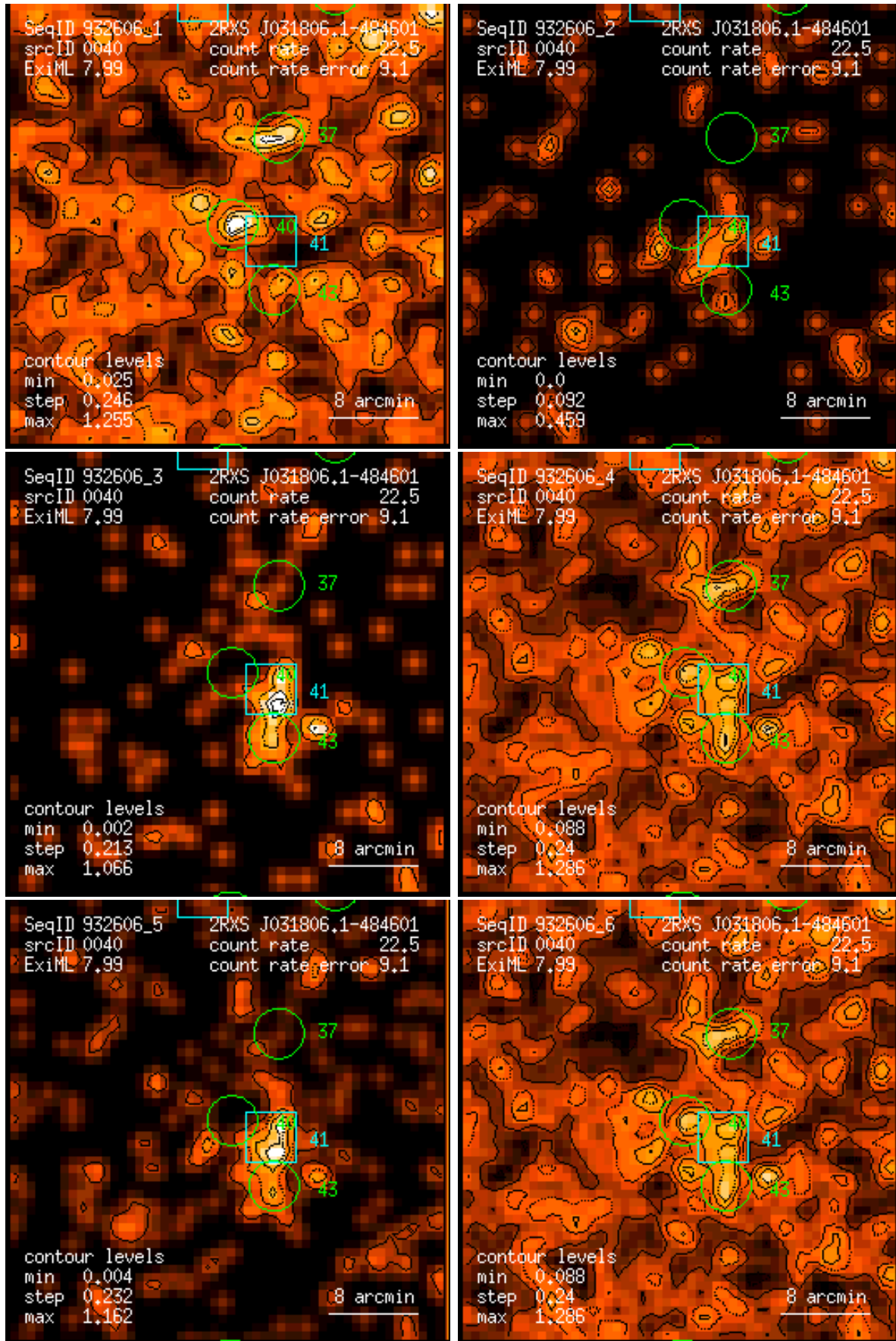
Figure 40: RASS 932606: detection 0040: band rate images, Gaussian filter: (1) PSPC channels 11 – 41, (2) 52 – 90, (3) 91 – 201, (4) 11 – 235, (5) 52 – 201, (6) 11 – 201. Broad band rates in counts/ks. Band rate contour levels in counts/ks/arcmin 2 .
