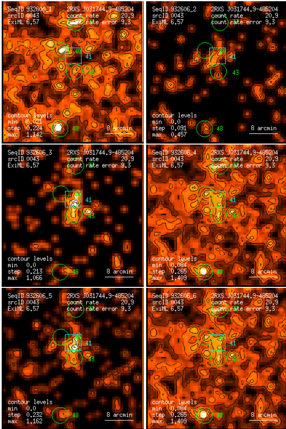
Figure 43: RASS 932606: detection 0043: band rate images, Gaussian filter: (1) PSPC channels 11 – 41, (2) 52 – 90, (3) 91 – 201, (4) 11 – 235, (5) 52 – 201, (6) 11 – 201. Broad band rates in counts/ks. Band rate contour levels in counts/ks/arcmin 2 .
