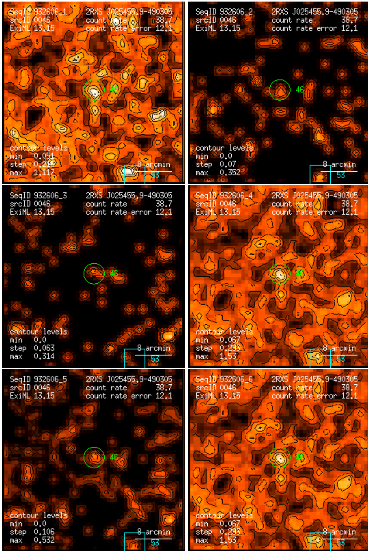
Figure 46: RASS 932606: detection 0046: band rate images, Gaussian filter: (1) PSPC channels 11 – 41, (2) 52 – 90, (3) 91 – 201, (4) 11 – 235, (5) 52 – 201, (6) 11 – 201. Broad band rates in counts/ks. Band rate contour levels in counts/ks/arcmin 2 .
