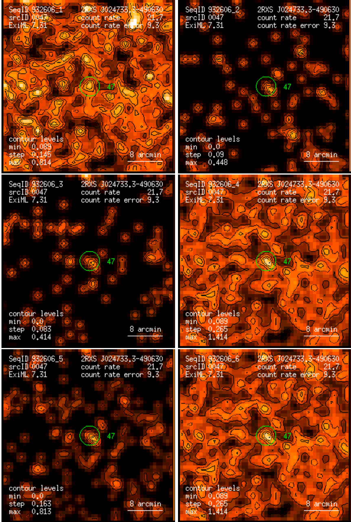
Figure 47: RASS 932606: detection 0047: band rate images, Gaussian filter: (1) PSPC channels 11 – 41, (2) 52 – 90, (3) 91 – 201, (4) 11 – 235, (5) 52 – 201, (6) 11 – 201. Broad band rates in counts/ks. Band rate contour levels in counts/ks/arcmin 2 .
