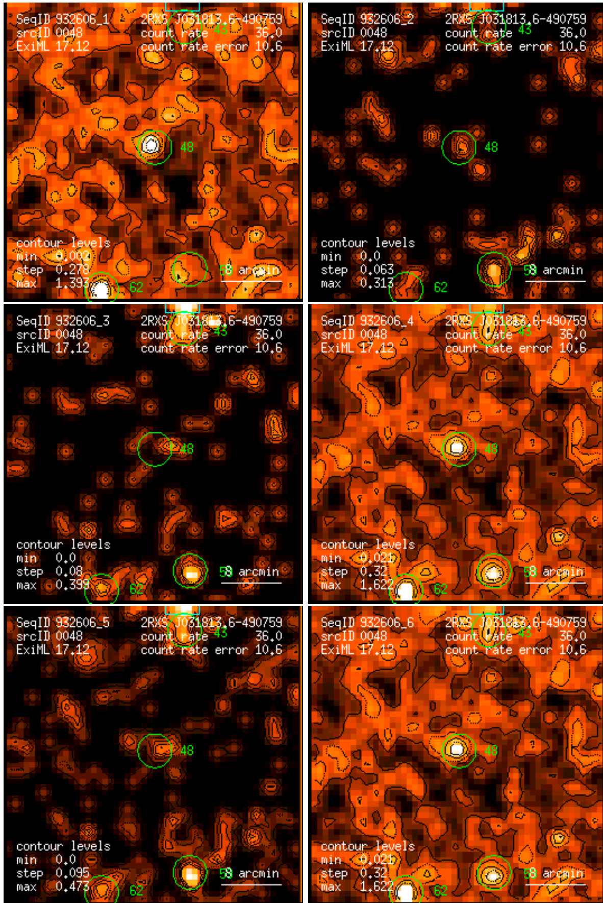
Figure 48: RASS 932606: detection 0048: band rate images, Gaussian filter: (1) PSPC channels 11 – 41, (2) 52 – 90, (3) 91 – 201, (4) 11 – 235, (5) 52 – 201, (6) 11 – 201. Broad band rates in counts/ks. Band rate contour levels in counts/ks/arcmin 2 .
