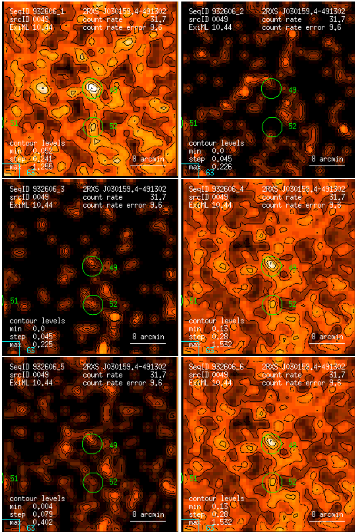
Figure 49: RASS 932606: detection 0049: band rate images, Gaussian filter: (1) PSPPC channels 11 – 41, (2) 52 – 90, (3) 91 – 201, (4) 11 – 235, (5) 52 – 201, (6) 11 – 201. Broad band rates in counts/ks. Band rate contour levels in counts/ks/arcmin 2 .
