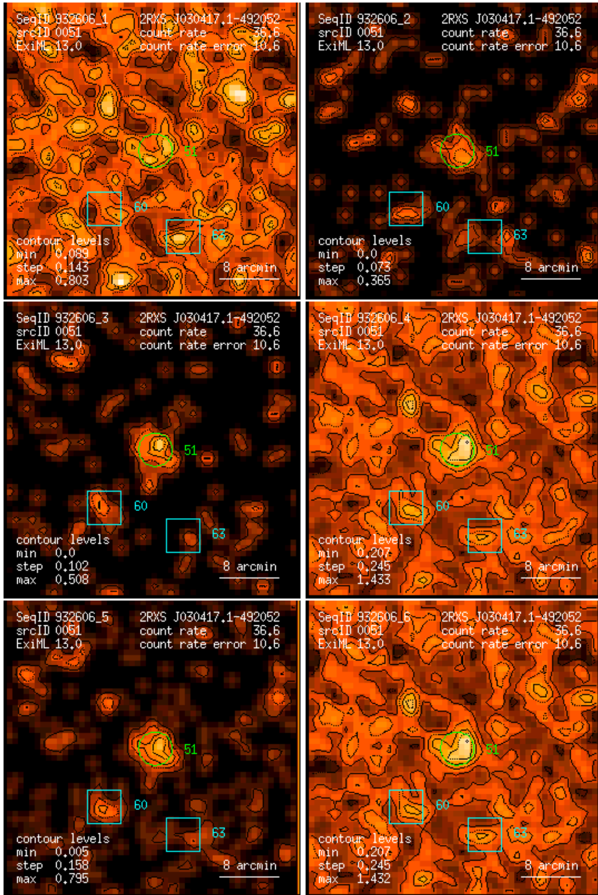
Figure 51: RASS 932606: detection 0051: band rate images, Gaussian filter: (1) PSPC channels 11 – 41, (2) 52 – 90, (3) 91 – 201, (4) 11 – 235, (5) 52 – 201, (6) 11 – 201. Broad band rates in counts/ks. Band rate contour levels in counts/ks/arcmin 2 .
