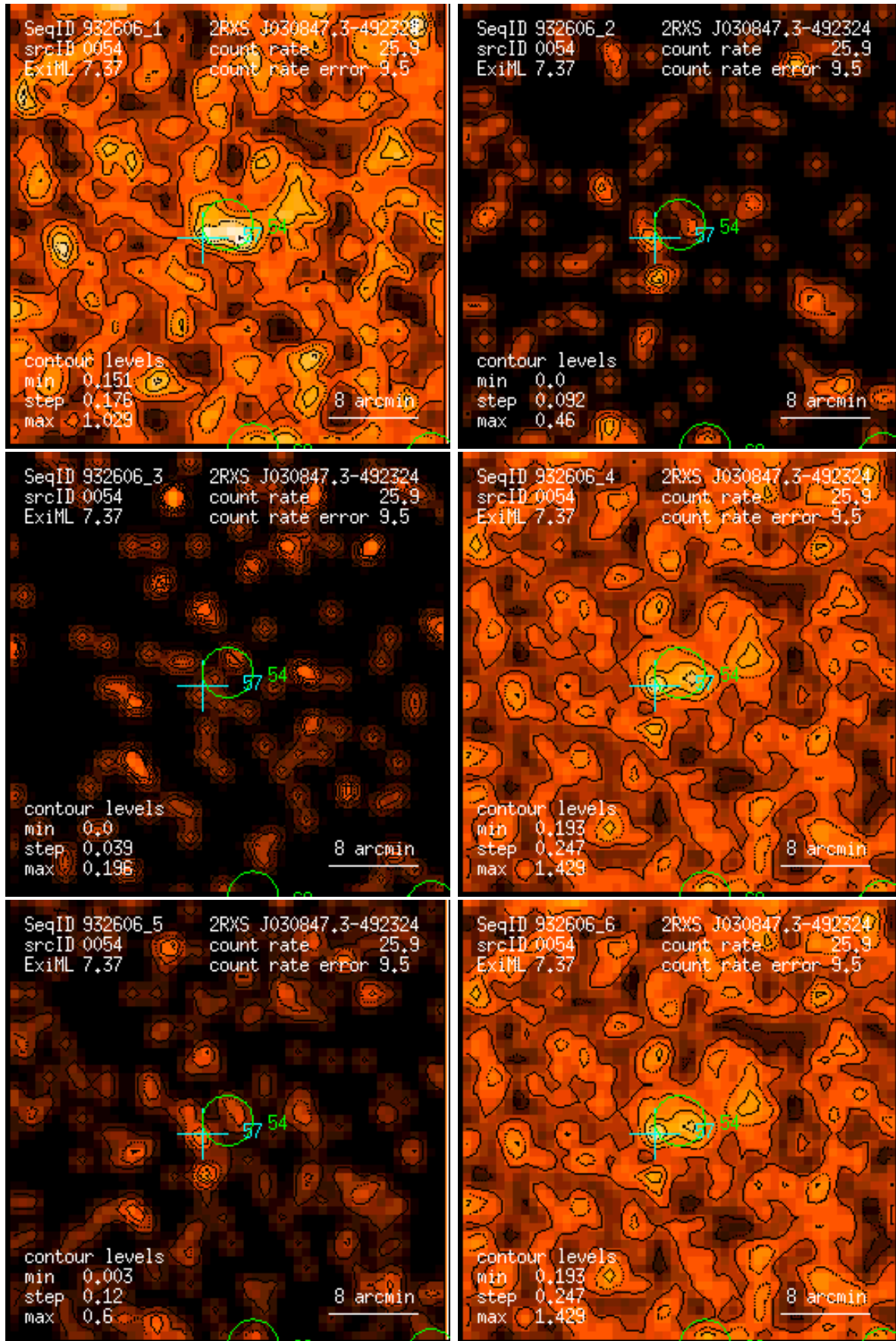
Figure 54: RASS 932606: detection 0054: band rate images, Gaussian filter: (1) PSPC channels 11 – 41, (2) 52 – 90, (3) 91 – 201, (4) 11 – 235, (5) 52 – 201, (6) 11 – 201. Broad band rates in counts/ks. Band rate contour levels in counts/ks/arcmin 2 .
