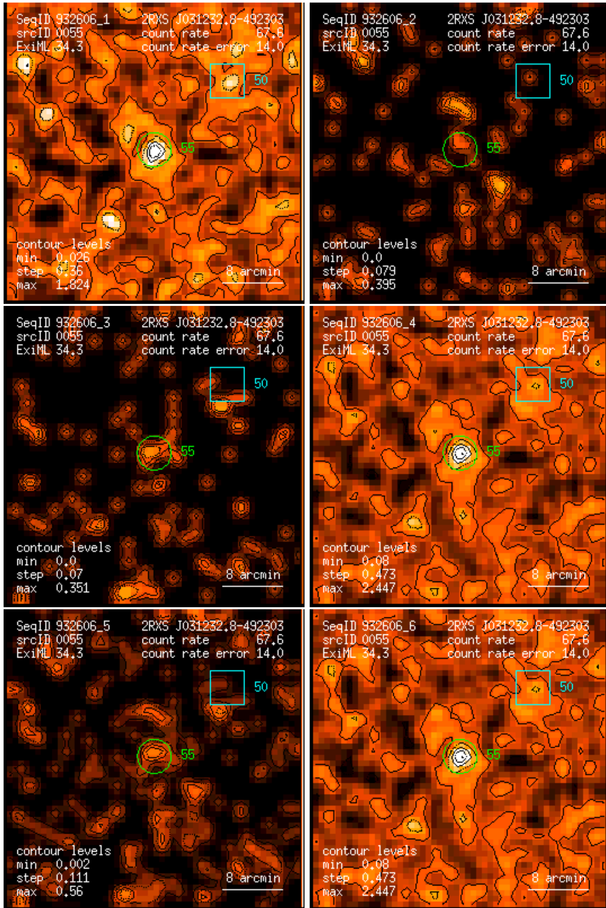
Figure 55: RASS 932606: detection 0055: band rate images, Gaussian filter: (1) PSPC channels 11 – 41, (2) 52 – 90, (3) 91 – 201, (4) 11 – 235, (5) 52 – 201, (6) 11 – 201. Broad band rates in counts/ks. Band rate contour levels in counts/ks/arcmin 2 .
