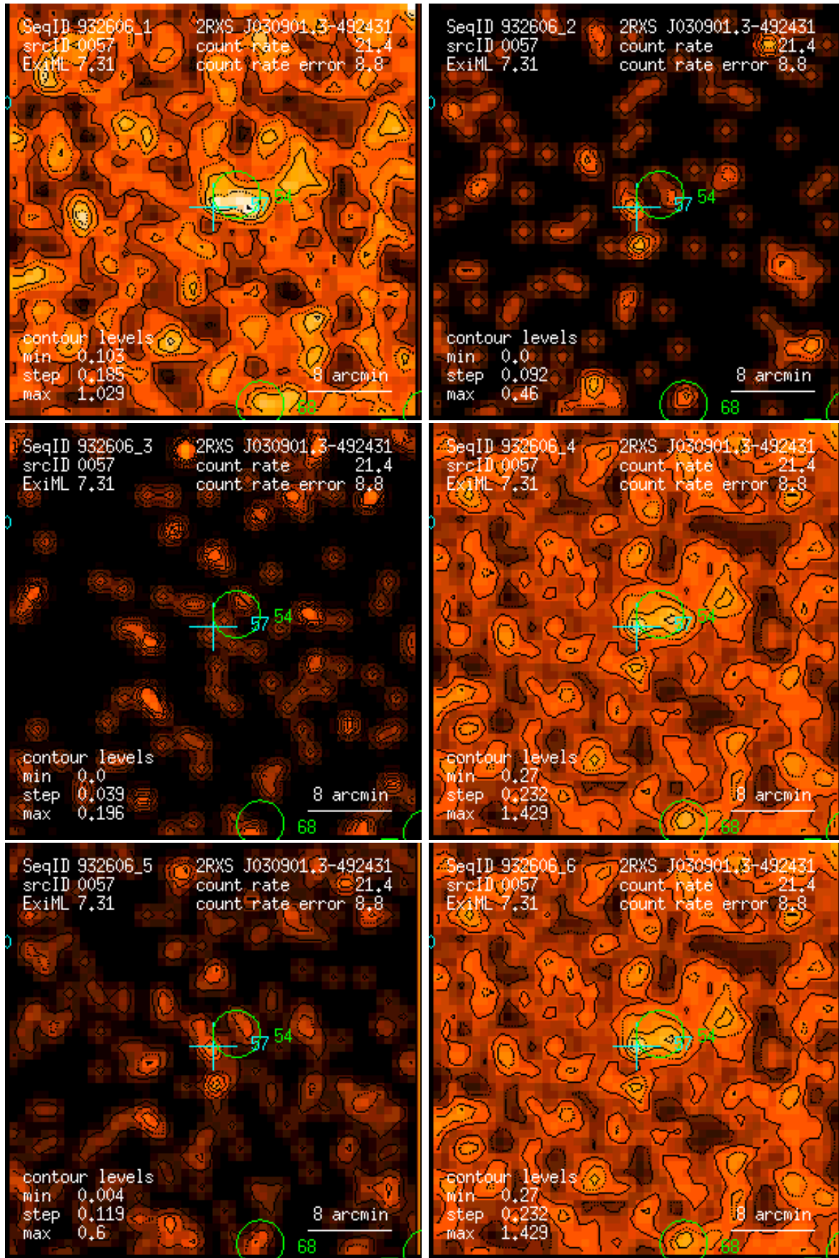
Figure 57: RASS 932606: detection 0057: band rate images, Gaussian filter: (1) PSPC channels 11 – 41, (2) 52 – 90, (3) 91 – 201, (4) 11 – 235, (5) 52 – 201, (6) 11 – 201. Broad band rates in counts/ks. Band rate contour levels in counts/ks/arcmin 2 .
