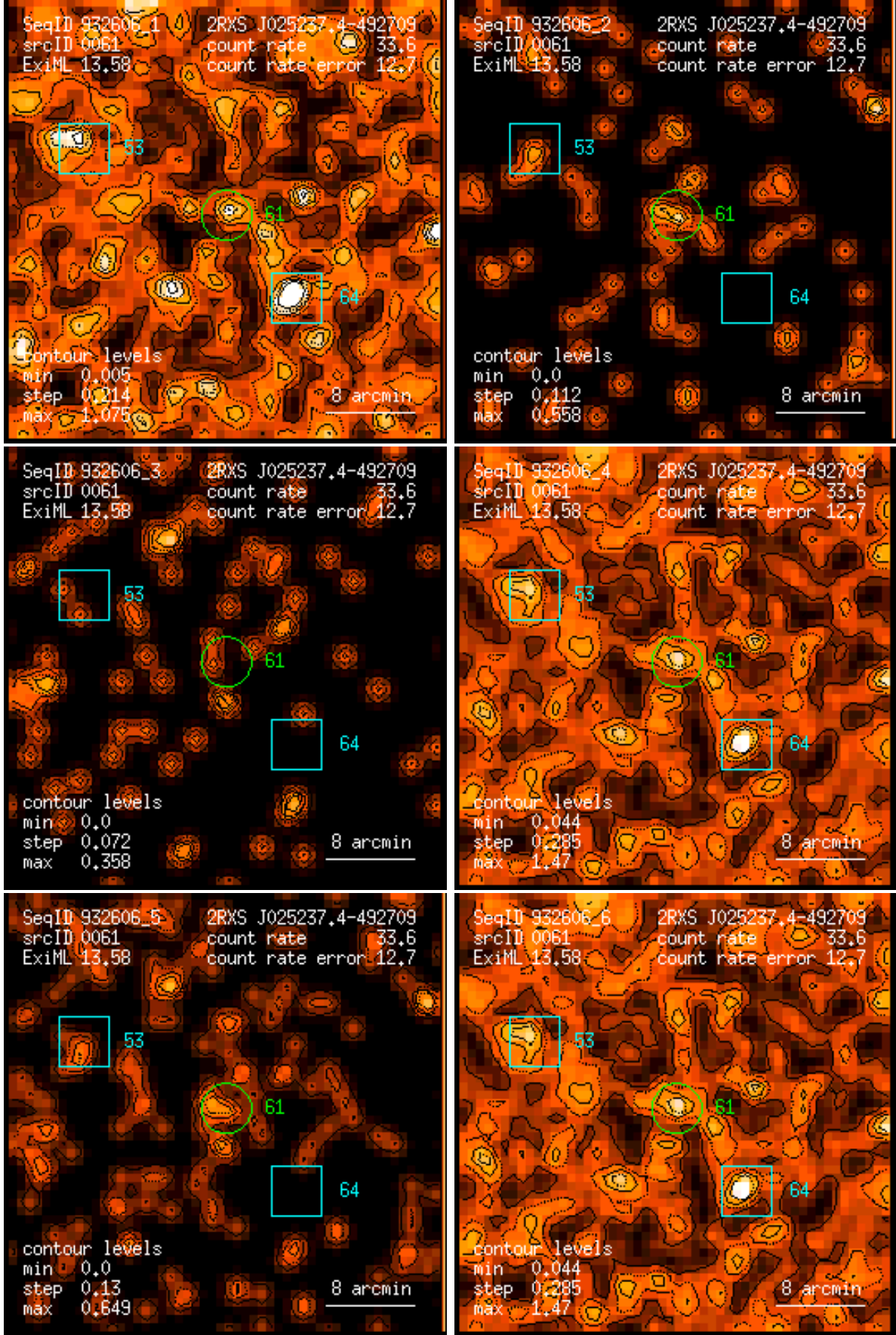
Figure 61: RASS 932606: detection 0061: band rate images, Gaussian filter: (1) PSPC channels 11 – 41, (2) 52 – 90, (3) 91 – 201, (4) 11 – 235, (5) 52 – 201, (6) 11 – 201. Broad band rates in counts/ks. Band rate contour levels in counts/ks/arcmin 2 .
