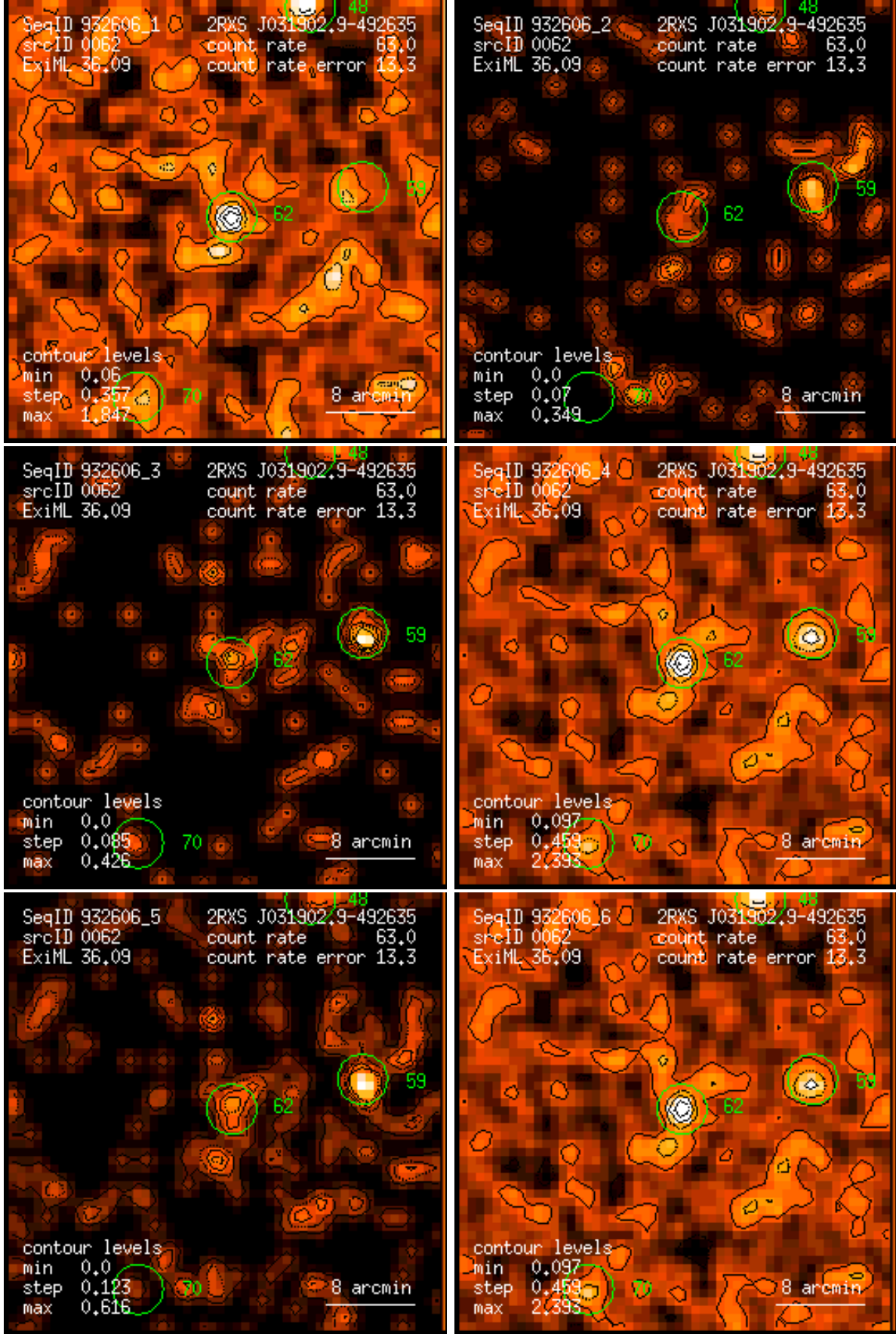
Figure 62: RASS 932606: detection 0062: band rate images, Gaussian filter: (1) PSPC channels 11 – 41, (2) 52 – 90, (3) 91 – 201, (4) 11 – 235, (5) 52 – 201, (6) 11 – 201. Broad band rates in counts/ks. Band rate contour levels in counts/ks/arcmin 2 .
