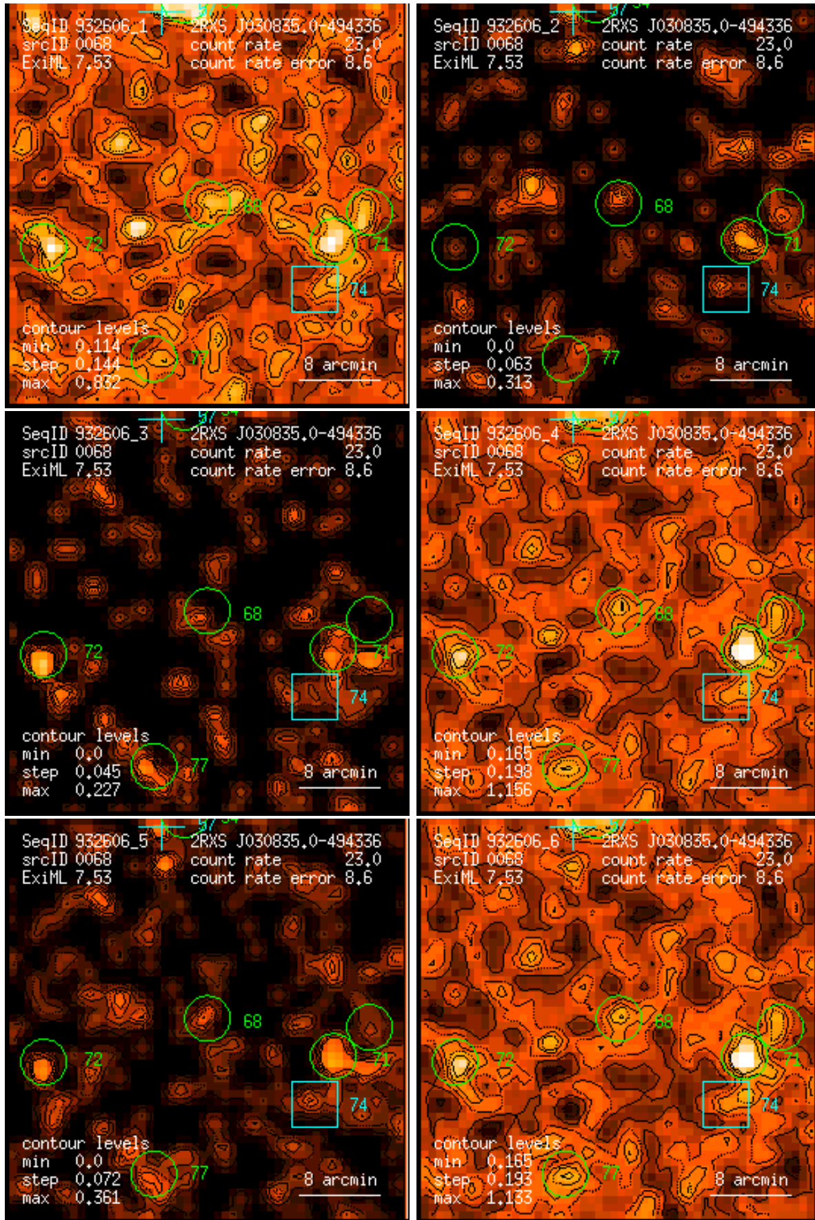
Figure 68: RASS 932606: detection 0068: band rate images, Gaussian filter: (1) PSPC channels 11 – 41, (2) 52 – 90, (3) 91 – 201, (4) 11 – 235, (5) 52 – 201, (6) 11 – 201. Broad band rates in counts/ks. Band rate contour levels in counts/ks/arcmin 2 .
