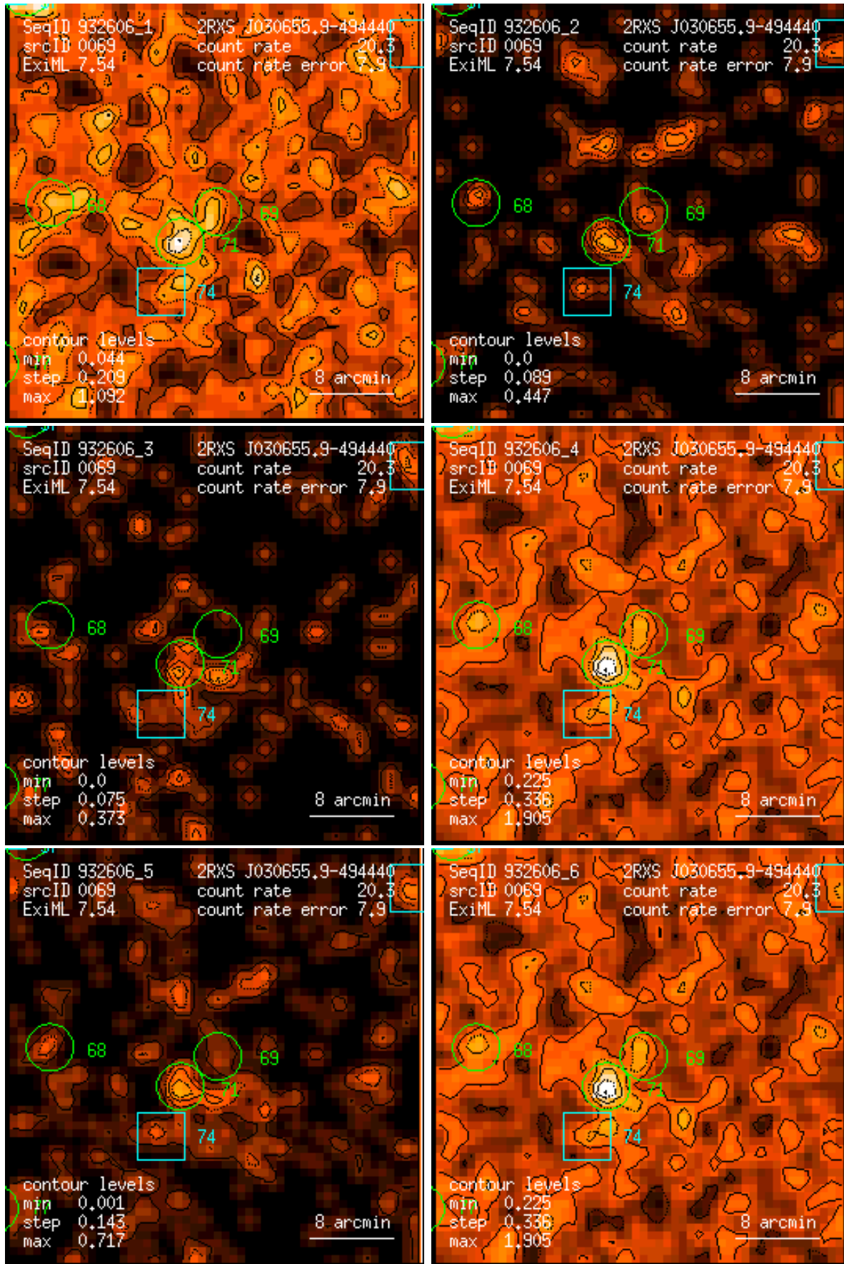
Figure 69: RASS 932606: detection 0069: band rate images, Gaussian filter: (1) PSPC channels 11 – 41, (2) 52 – 90, (3) 91 – 201, (4) 11 – 235, (5) 52 – 201, (6) 11 – 201. Broad band rates in counts/ks. Band rate contour levels in counts/ks/arcmin 2 .
