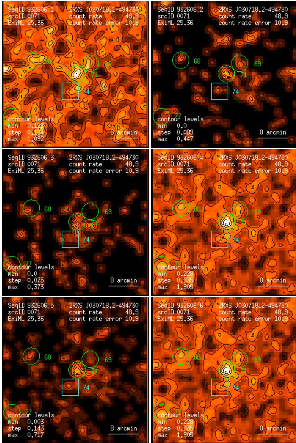
Figure 71: RASS 932606: detection 0071: band rate images, Gaussian filter: (1) PSPC channels 11 – 41, (2) 52 – 90, (3) 91 – 201, (4) 11 – 235, (5) 52 – 201, (6) 11 – 201. Broad band rates in counts/ks. Band rate contour levels in counts/ks/arcmin 2 .
